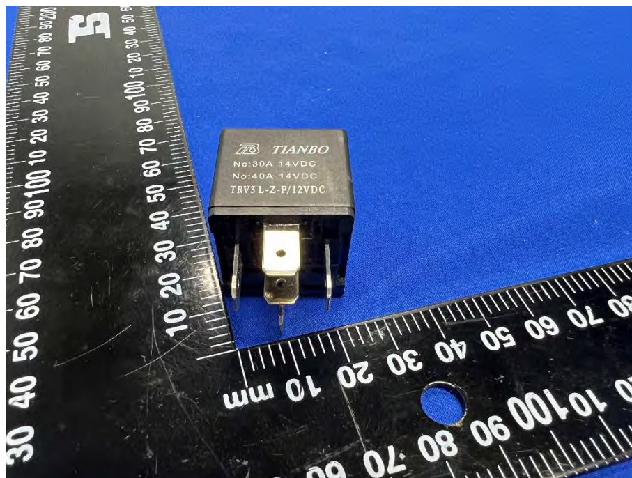
Accessory-Relay(12V/24V)
