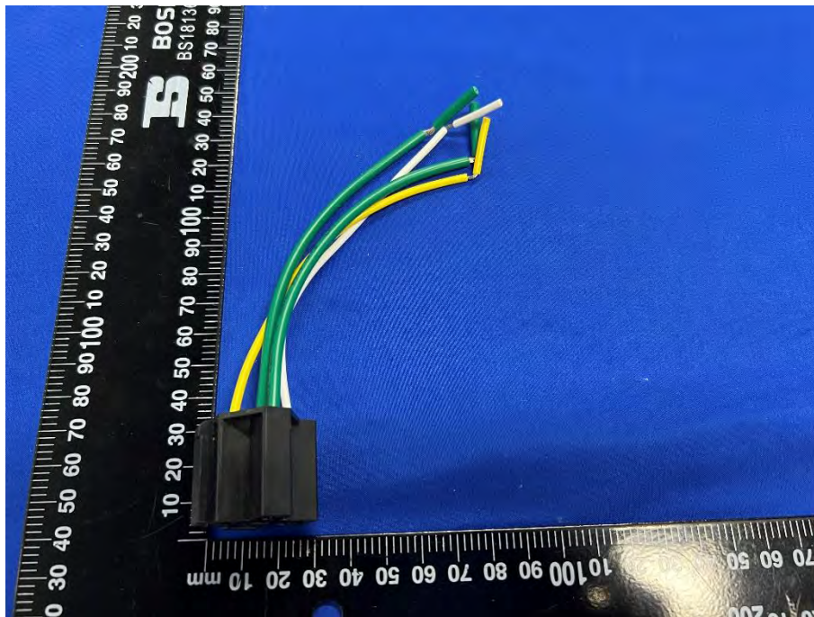
Accessory-Relay cable
