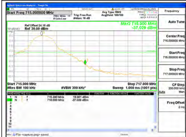
Band17 / 10MHz / High CH / QPSK / 1 RB
