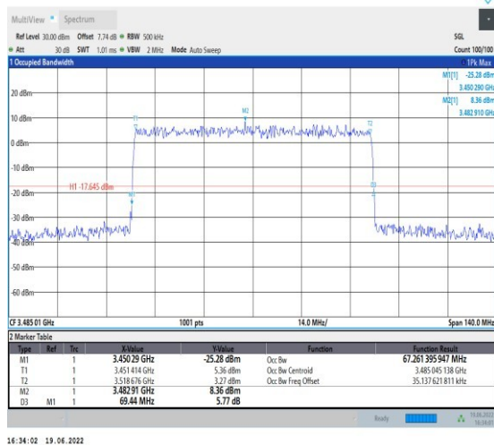
1-N78-3450-3550-PC2-30-70-L-9-CP-256QAM-Outer _Full-189@0-Ant1-67.261-69.440-≤70-PASS
