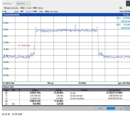
1-N78-3450-3550-PC2-30-70-L-7-CP-16QAM-Outer _Full-189@0-Ant1-67.293-70.000-≤70-PASS
