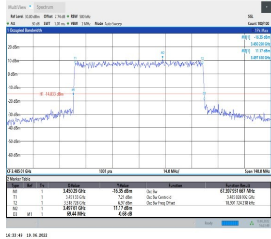
1-N78-3450-3550-PC2-30-70-L-8-CP-64QAM-Outer _Full-189@0-Ant1-67.398-69.440-≤70-PASS
