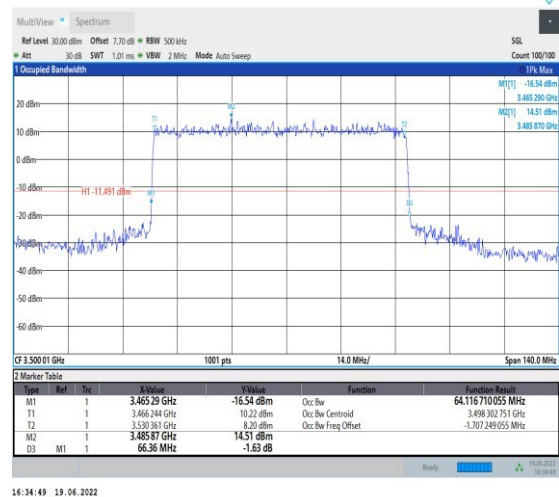
1-N78-3450-3550-PC2-30-70-M-1-DFT-QPSK-Outer _Full-180@0-Ant1-64.117-66.360-≤70-PASS
