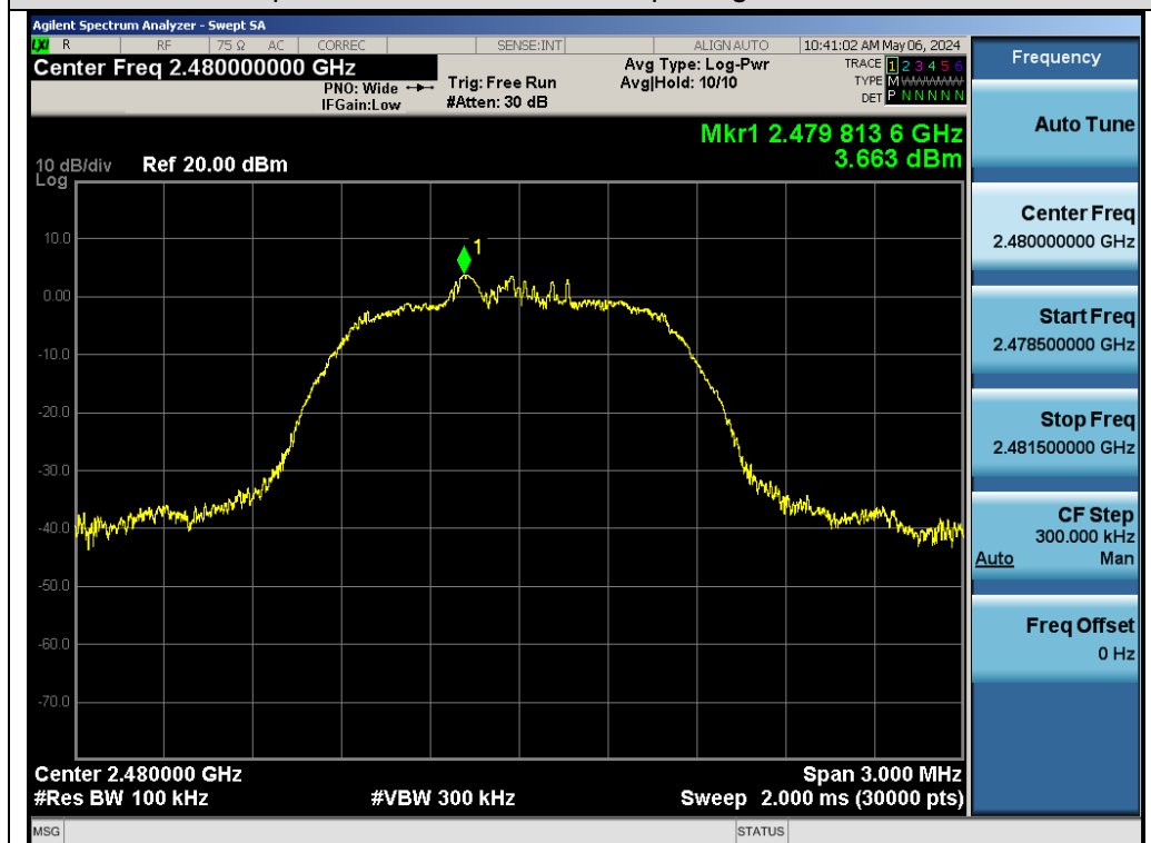
Test Graph EDR ANT1 2480 2Mbps Reference Level
