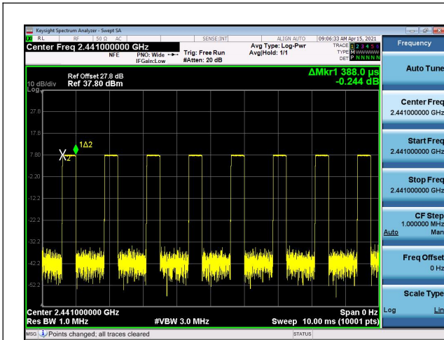
Modulation: GFSK DH1 2441
