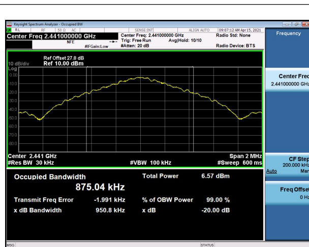
Modulation: GFSK 2441MHz
