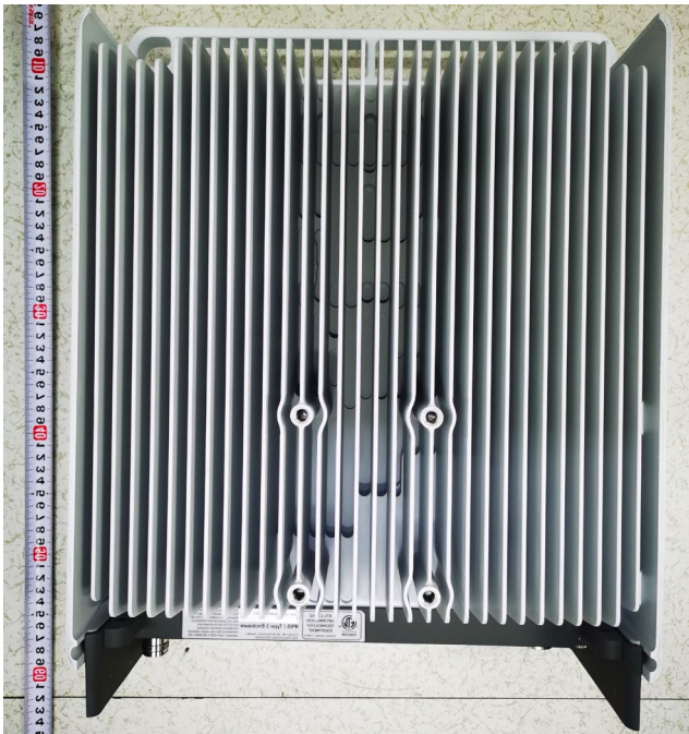
Rear side
