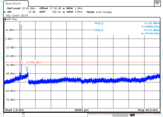
11AC20MIMO-Ant2-5260-1000~40000-PASS
