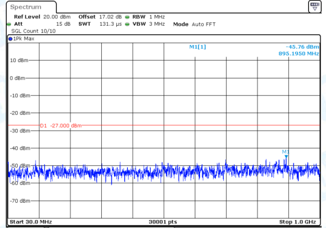
11N40MIMO-Ant2-5310-30~1000-PASS
