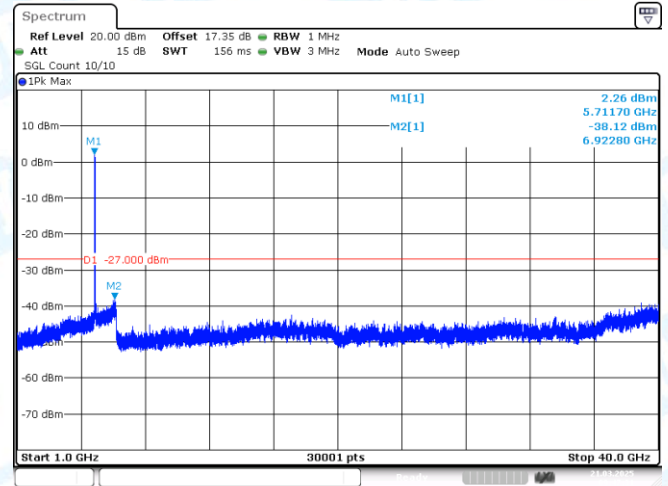
11N40MIMO-Ant2-5710-1000~40000-PASS
