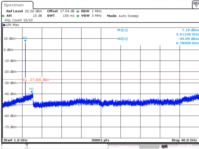
11N40MIMO-Ant1-5510-1000~40000-PASS
