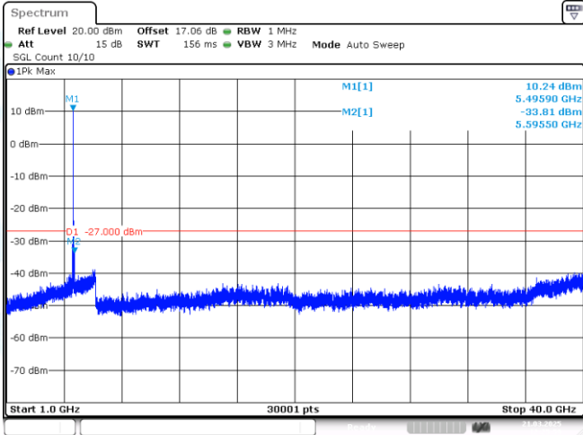
11AC20MIMO-Ant1-5500-1000~40000-PASS
