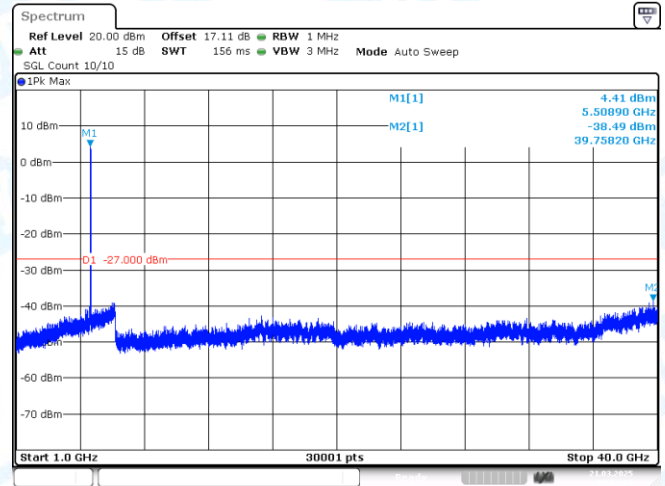
11N40MIMO-Ant2-5510-1000~40000-PASS
