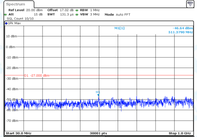
11AC20MIMO-Ant2-5320-30~1000-PASS
