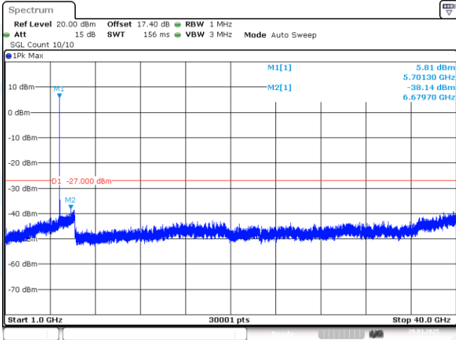
11N20MIMO-Ant1-5700-1000~40000-PASS
