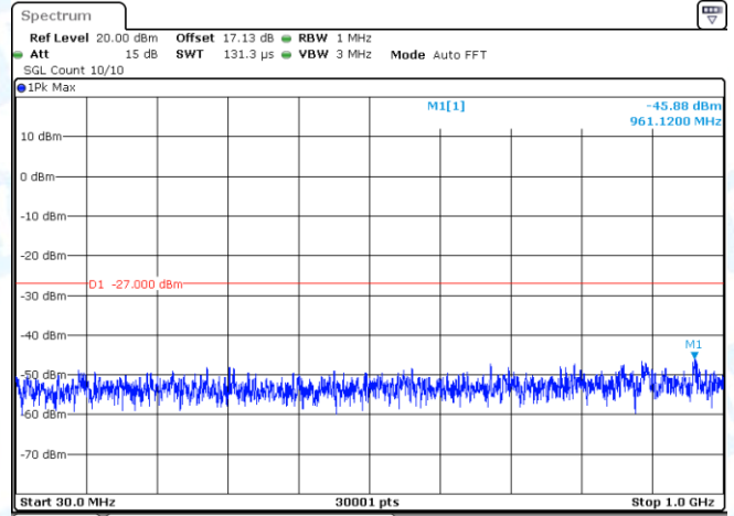
11N20MIMO-Ant2-5580-30~1000-PASS
