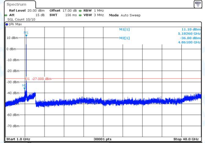
11AC20MIMO-Ant2-5180-1000~40000-PASS
