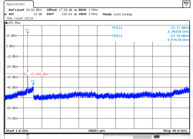
11N20MIMO-Ant2-5785-1000~40000-PASS
