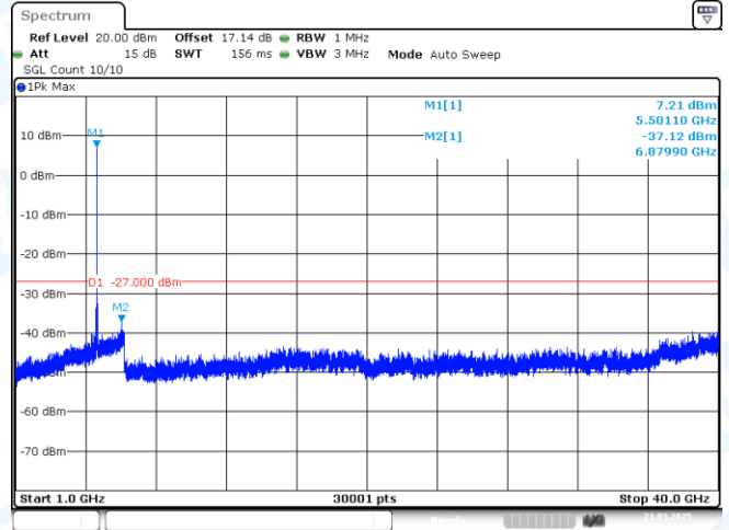
11AC20MIMO-Ant2-5500-1000~40000-PASS
