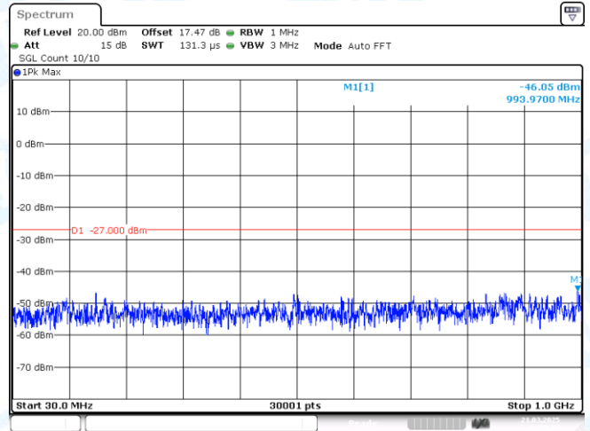
11N40MIMO-Ant2-5670-30~1000-PASS
