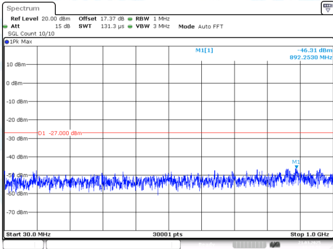
11N40MIMO-Ant1-5670-30~1000-PASS
