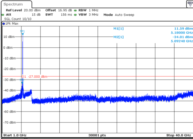
11AC20MIMO-Ant1-5180-1000~40000-PASS
