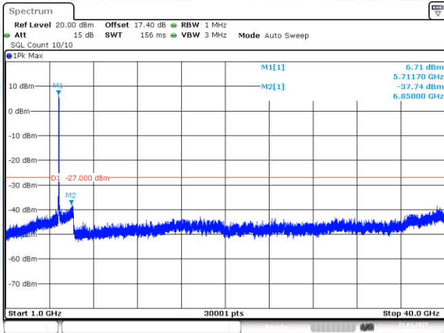
11N40MIMO-Ant1-5710-1000~40000-PASS
