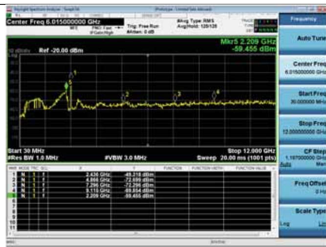
Antenna D
