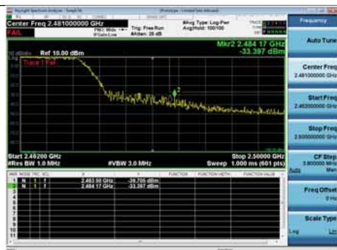
Antenna D
