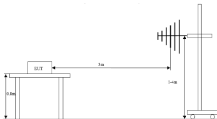
(Radiated emission)
