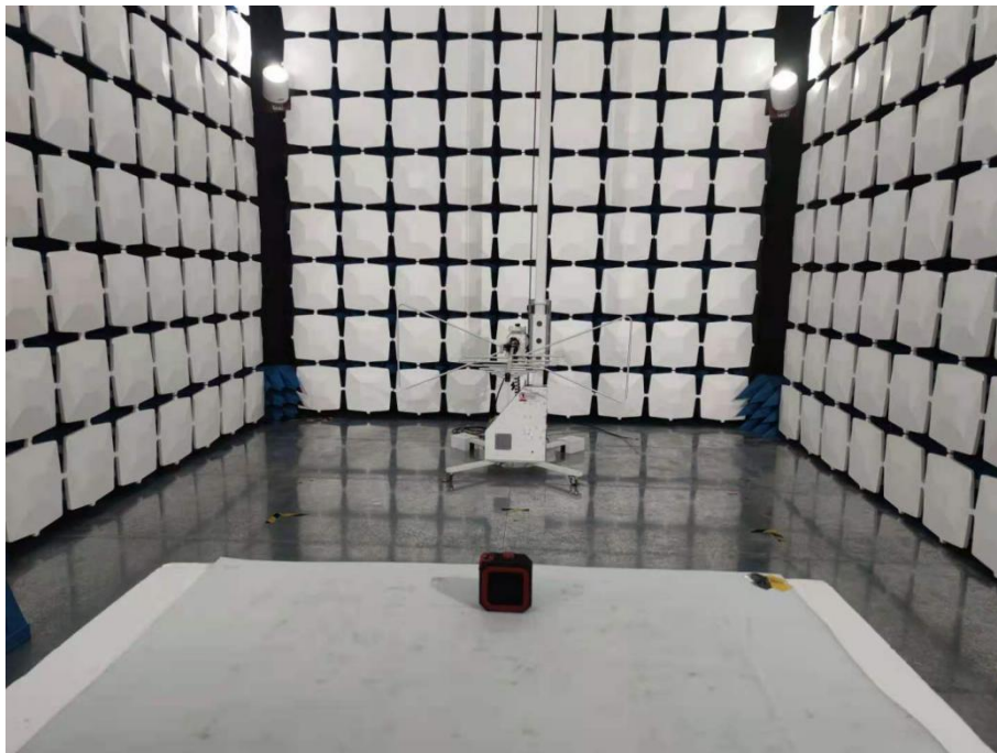
Blow 1GHz for radiated emission test setup
