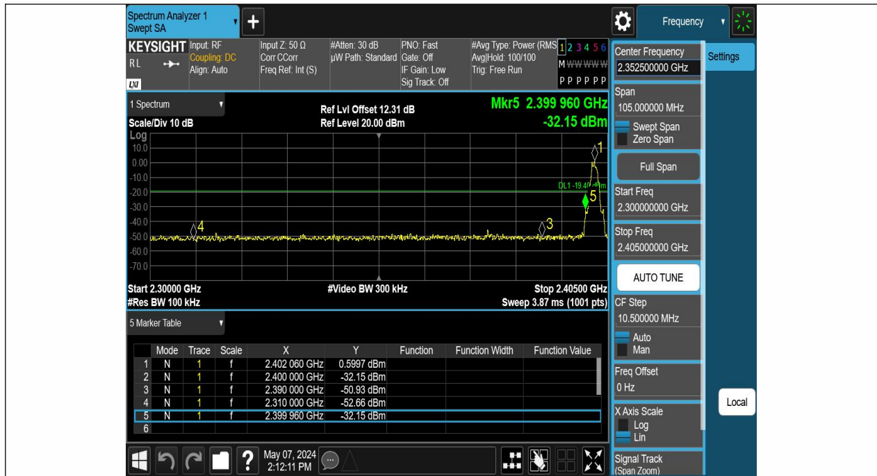
BLE_2M-Ant1-2402-PASS
