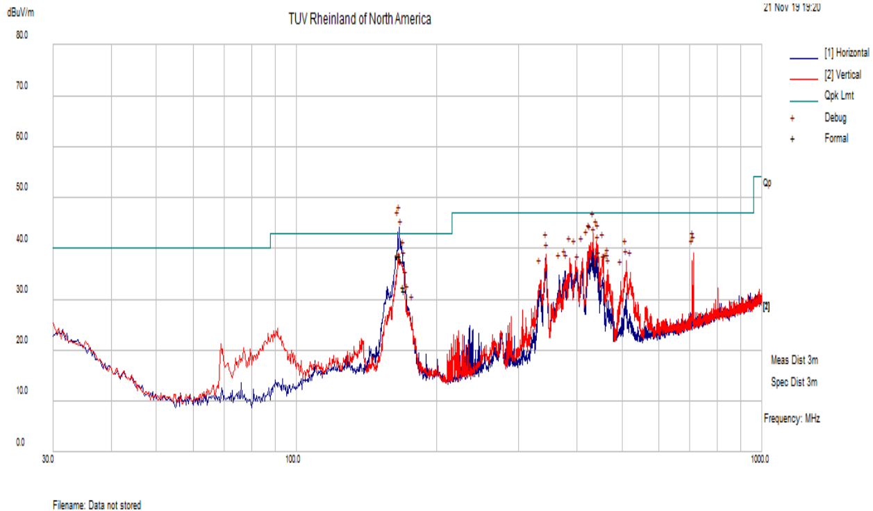
Radiated Emissions 30-1000 MHz.
