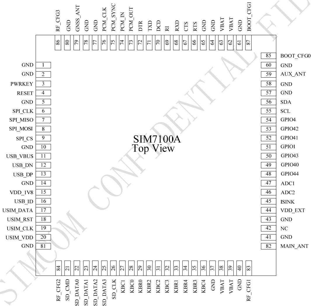
Figure 2: Pin view
