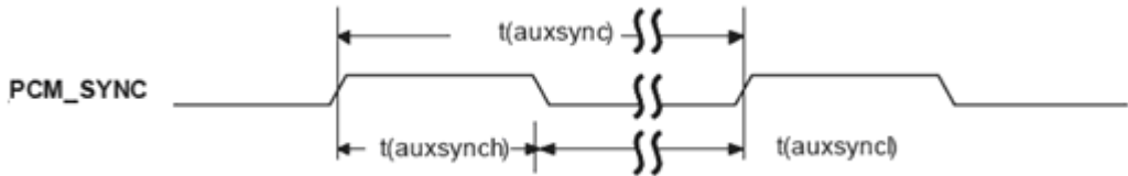
Figure 21: Synchrony timing
