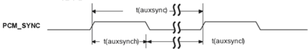
Figure 24: Synchrony timing
