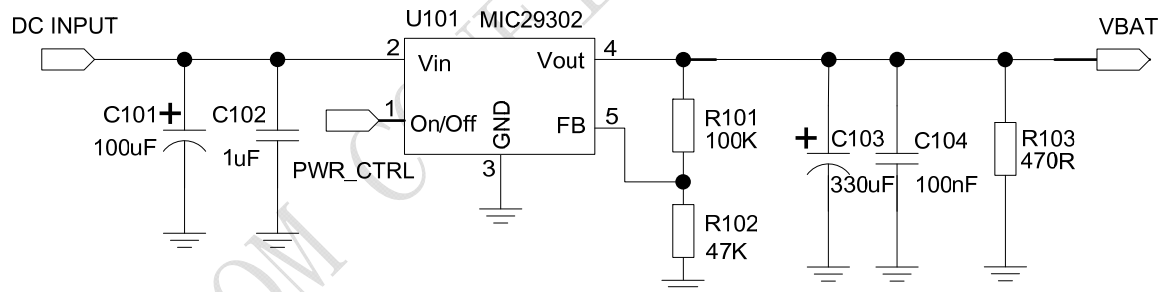
Figure 8: Reference circuit of the LDO power supply
