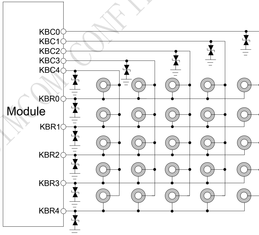
Figure 29: Reference circuit
