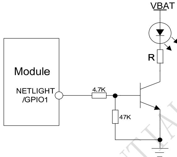
Figure 30: Application circuit
