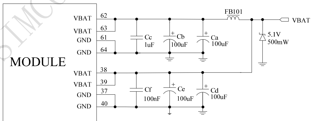
Figure 7: VBAT input application circuit
