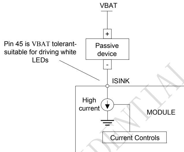
Figure 32: Current drive
