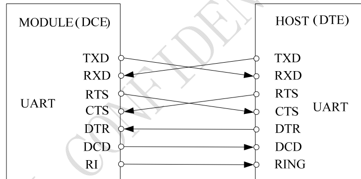
Figure 15: UART Full modem
