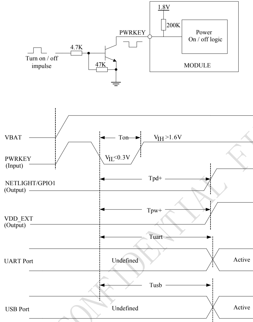
Figure 10: Power on Timing Sequence
