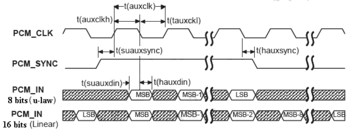
Figure 22: EXT CODEC to MODULE timing
