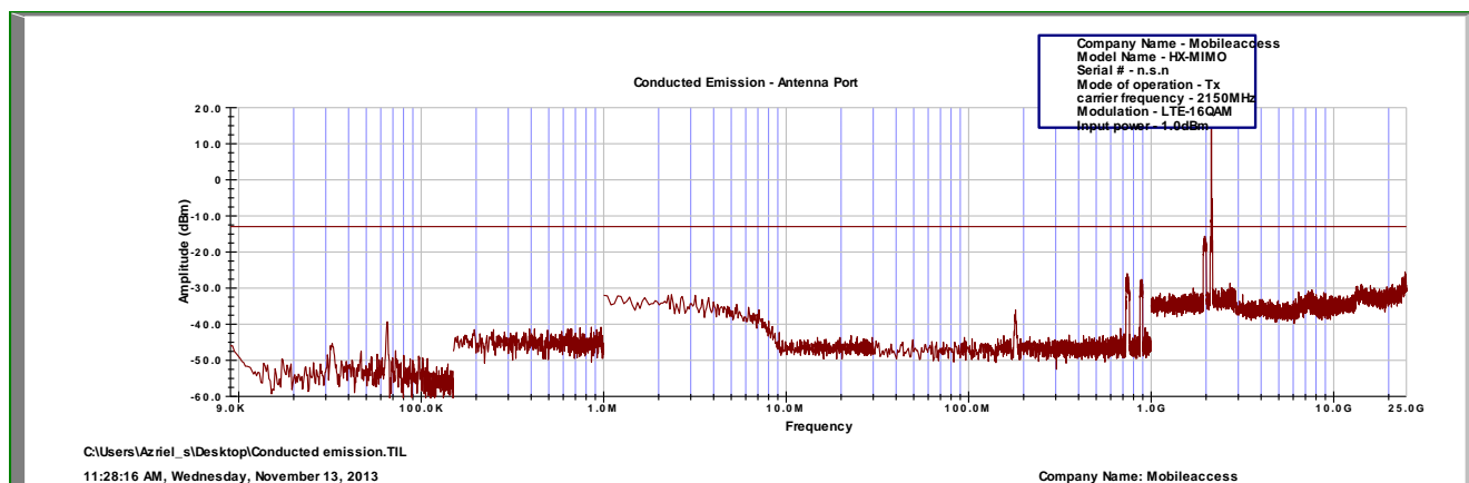
Figure 40.— 16QAM (High)
