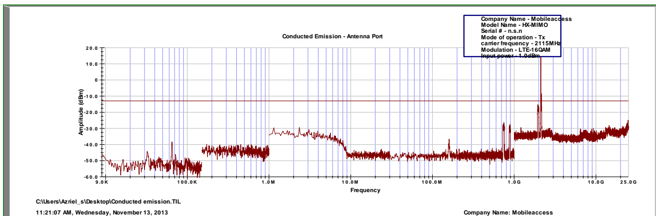
Figure 38.— 16QAM (Low)
