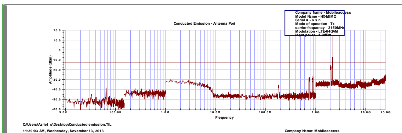
Figure 42.— 64QAM (Mid)
