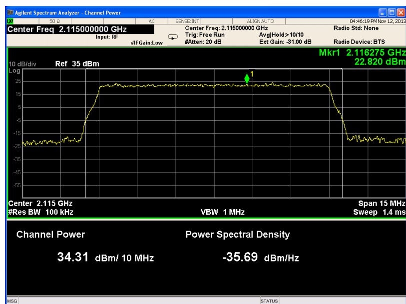
Figure 13 - QPSK (LOW)
