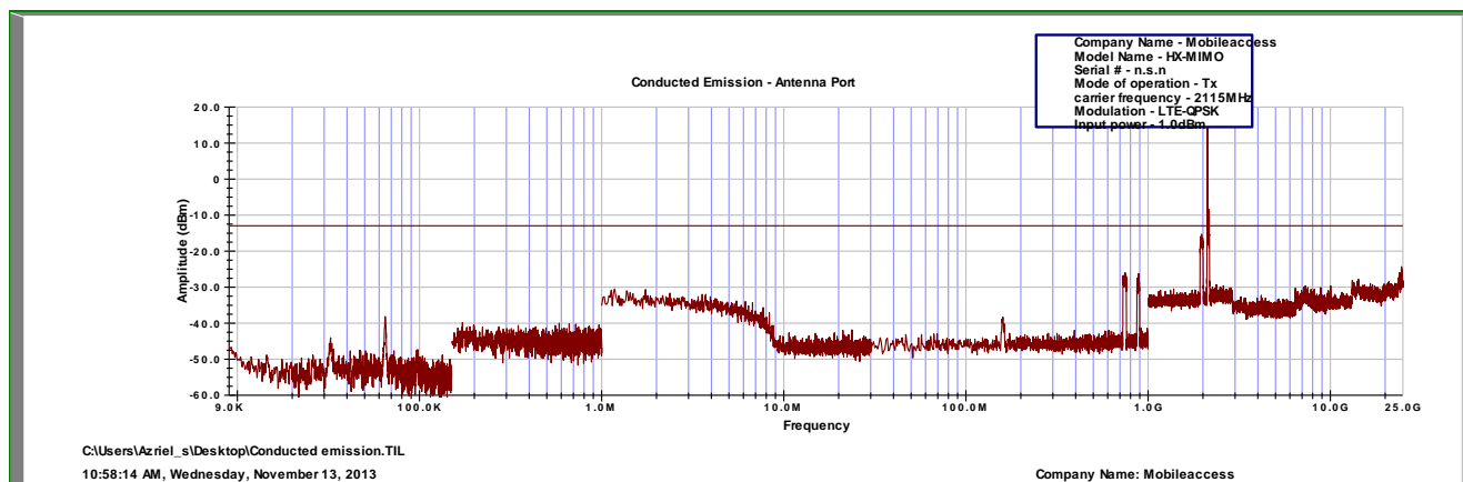
Figure 44.— QPSK (Low)
