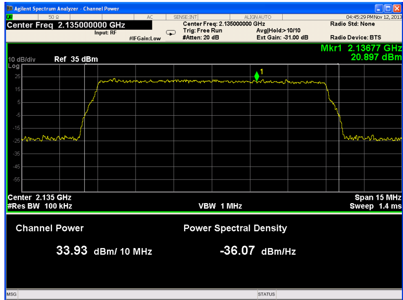
Figure 14 - QPSK (MID)
