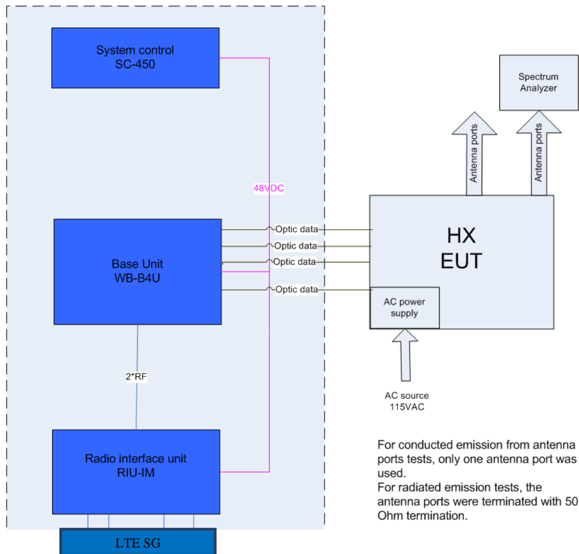
Figure 1. Test Set-up
