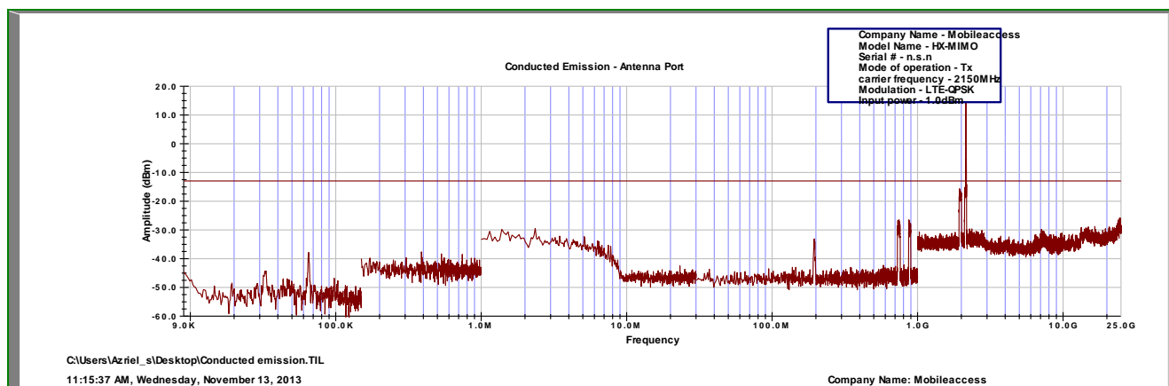
Figure 46.— QPSK (High)
