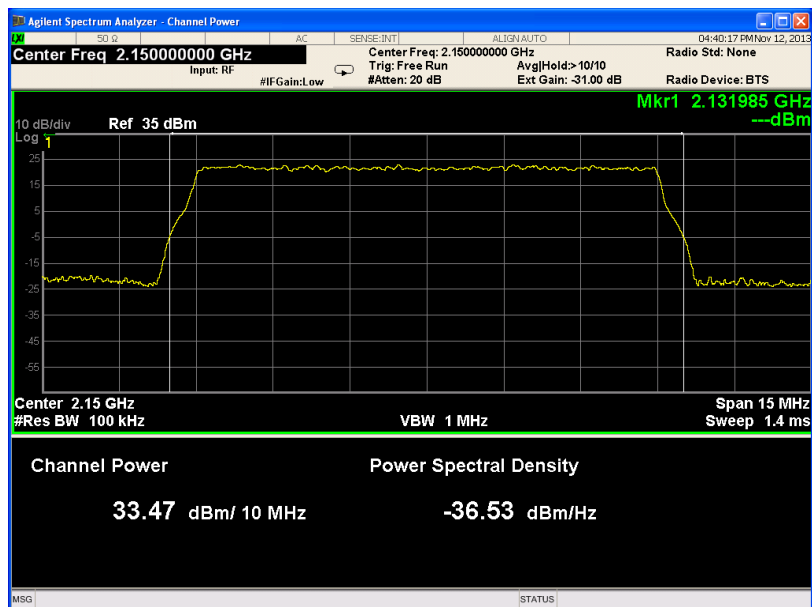
Figure 9 - 16QAM (HIGH)
