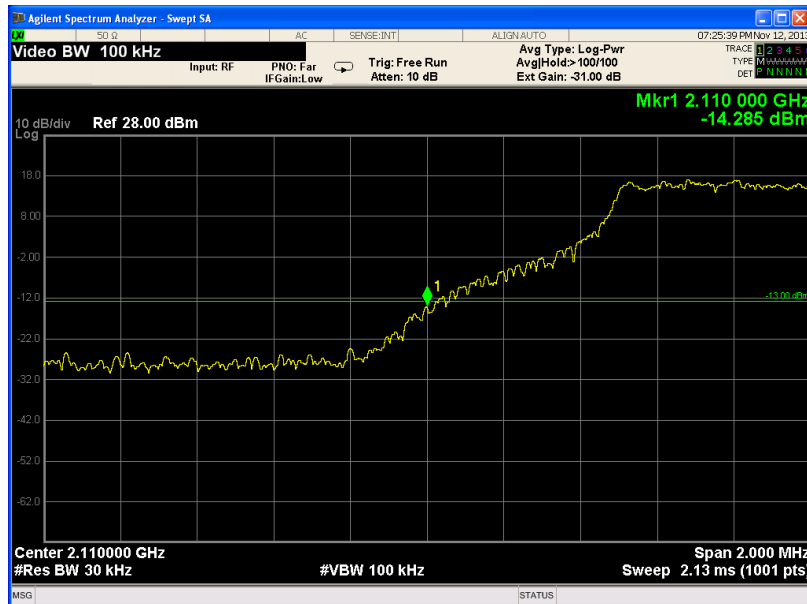
Figure 50.— 64QAM LOW
