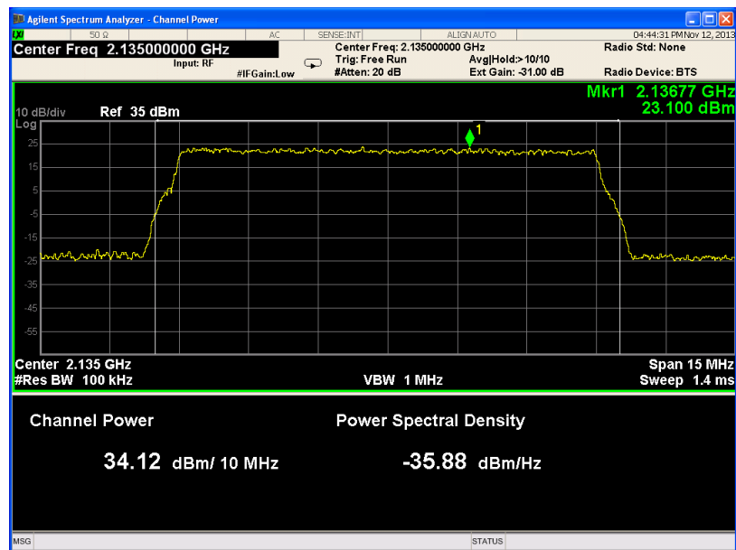
Figure 8 - 16QAM (MID)
