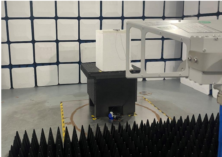
Above 1GHz
