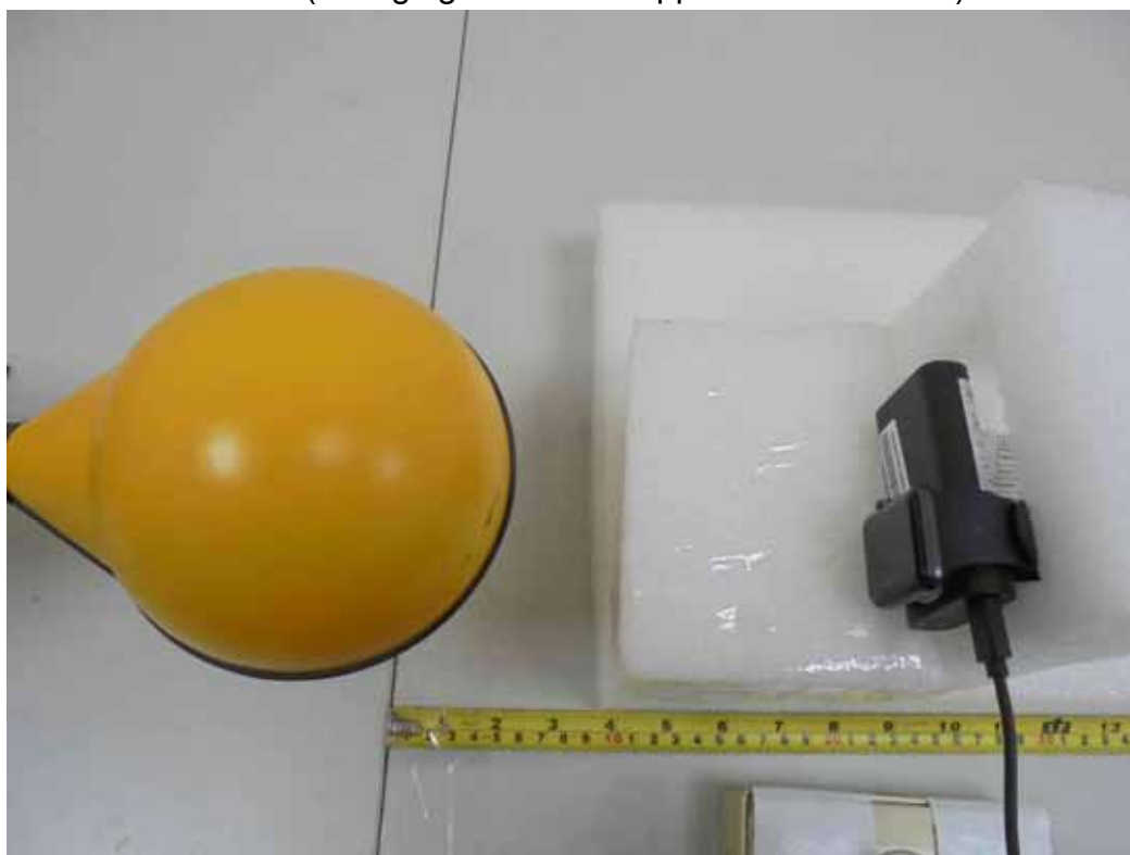
H-Field (Charging Mode with Apple Watch - Z-axis)
