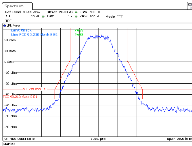
Plot 7.3.2 Emission mask test results at mid carrier frequency FCC part 90
