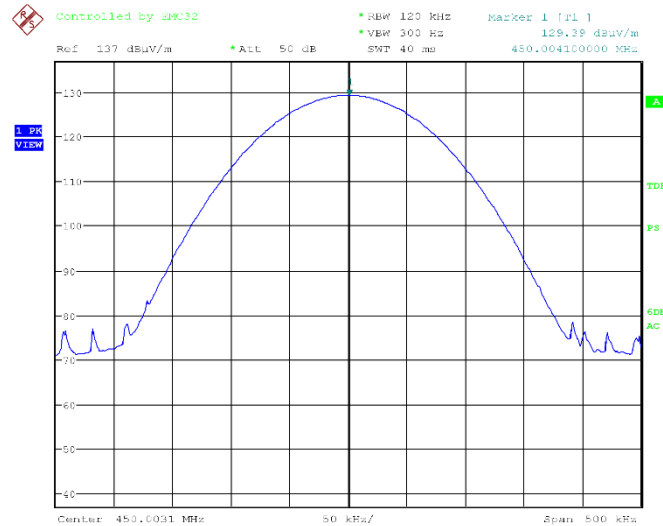
Plot 7.1.1 Transmitter carrier field strength at low frequency in vertical and horizontal antenna polarization
