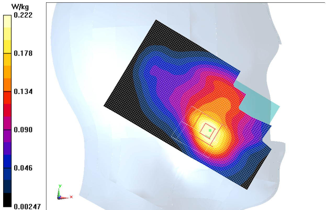
Fig.I.3 1900 MHz CH810
