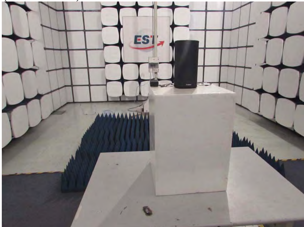
Radiated Test (Above 1000 MHz)
