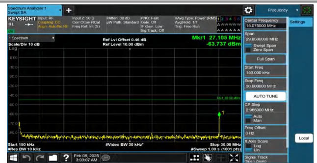
Band38-15MHz-QPSK-38000-1RB#0-0.15~30-PASS
