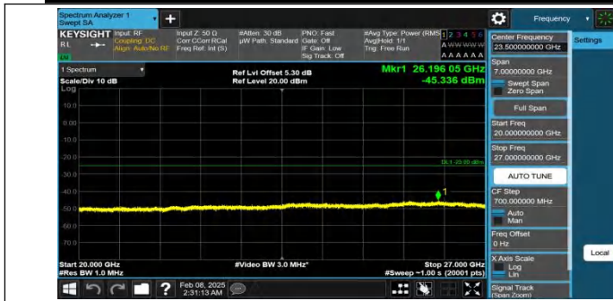
Band38-5MHz-QPSK-38225-1RB#0-20000~27000-PASS
