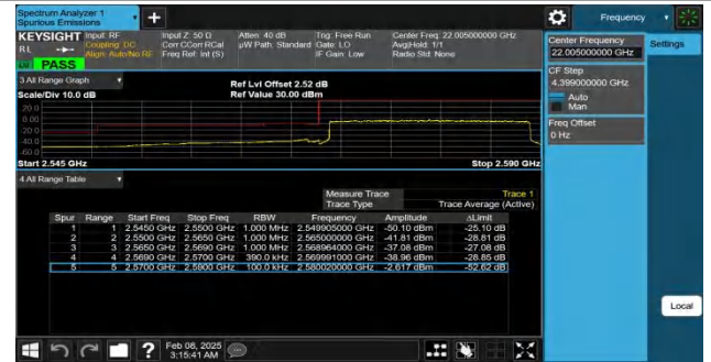
Band38-20MHz-QPSK-37850-100RB#0-PASS
