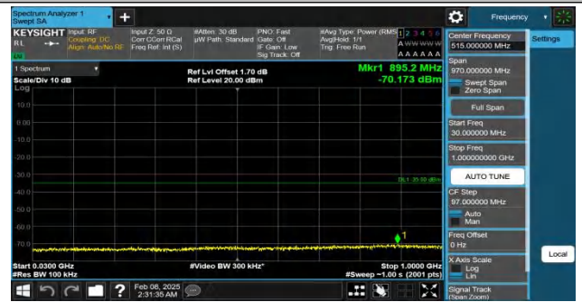
Band38-5MHz-QPSK-38225-1RB#24-30~1000-PASS
