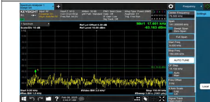
Band38-10MHz-QPSK-37800-1RB#0-0.009~0.15-PASS
