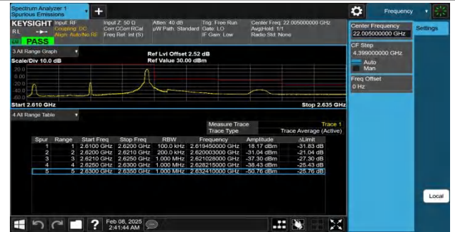
Band38-10MHz-QPSK-38200-1RB#49-PASS
