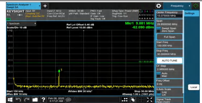
Band38-20MHz-QPSK-37850-1RB#0-0.15~30-PASS
