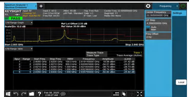
Band38-15MHz-QPSK-38175-1RB#74-PASS
