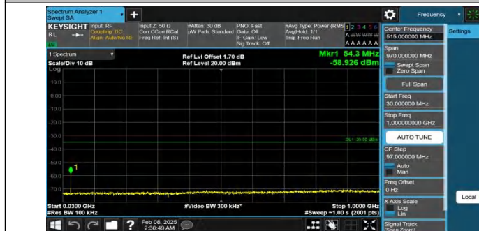
Band38-5MHz-QPSK-38225-1RB#0-30~1000-PASS
