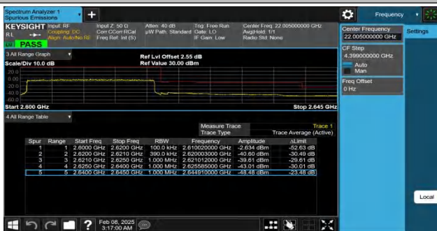
Band38-20MHz-QPSK-38150-100RB#0-PASS
