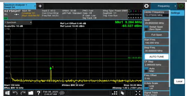
Band38-10MHz-QPSK-37800-1RB#0-0.15~30-PASS
