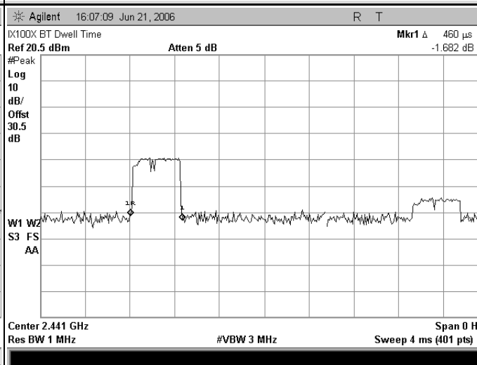
Figure E.8-2 - Pulse Width
