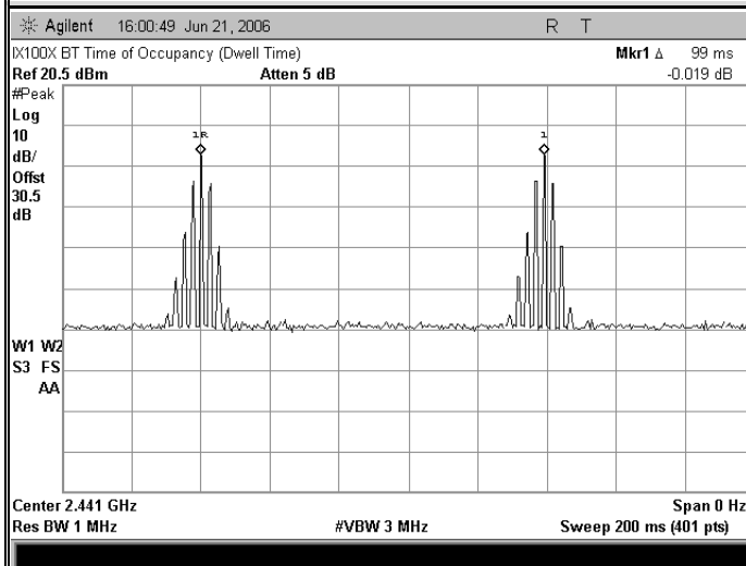
Figure E.8-1 - List Repetition Rate
