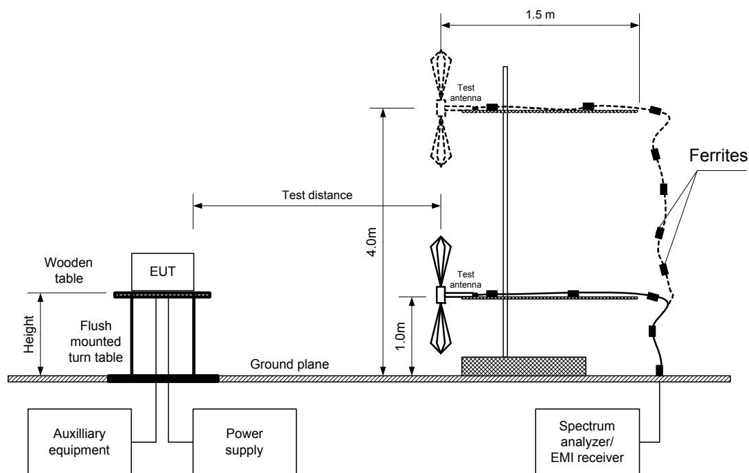
Figure 7.5.1 Setup for carrier field strength measurements
