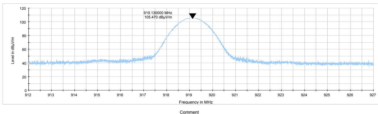
Plot 7.5.3 Field strength of carrier at high frequency
