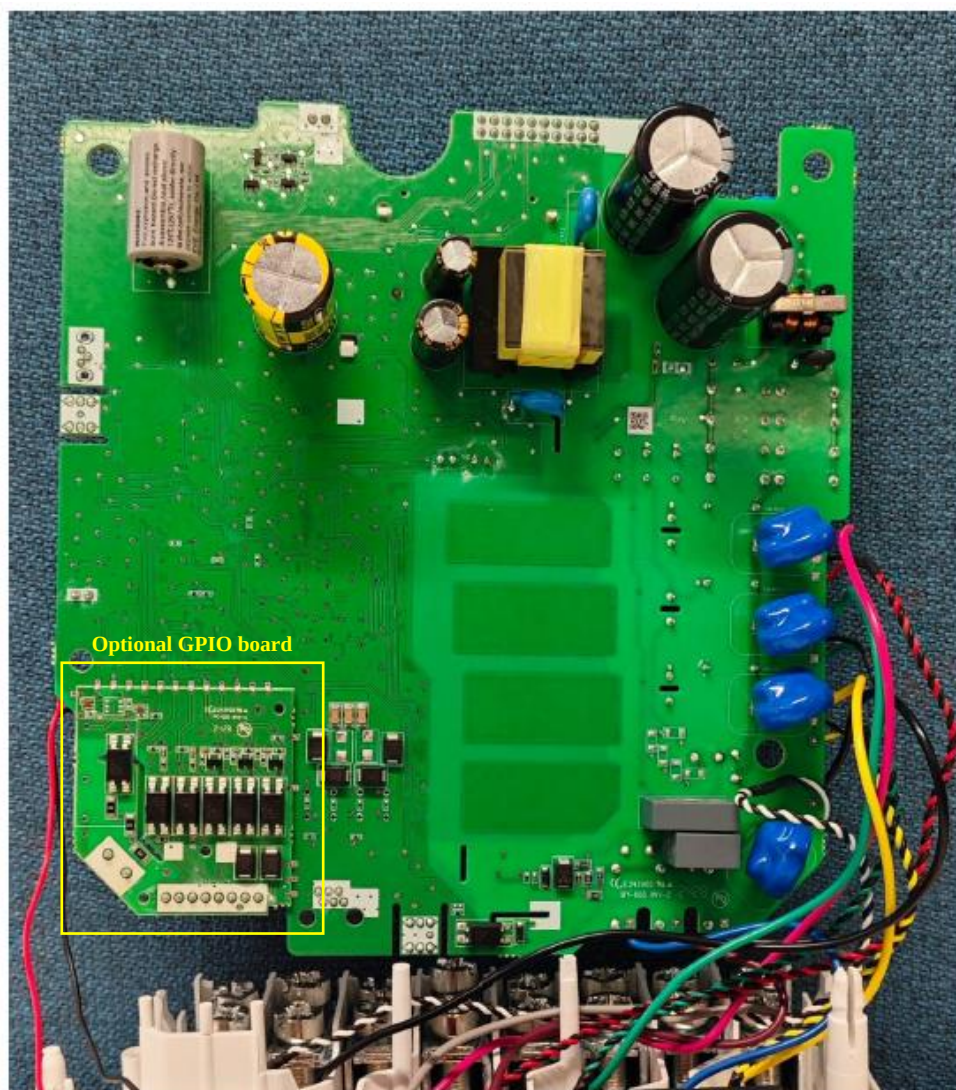
Figure 4 – GLOBYTGNG3 bottom PCB view full version
