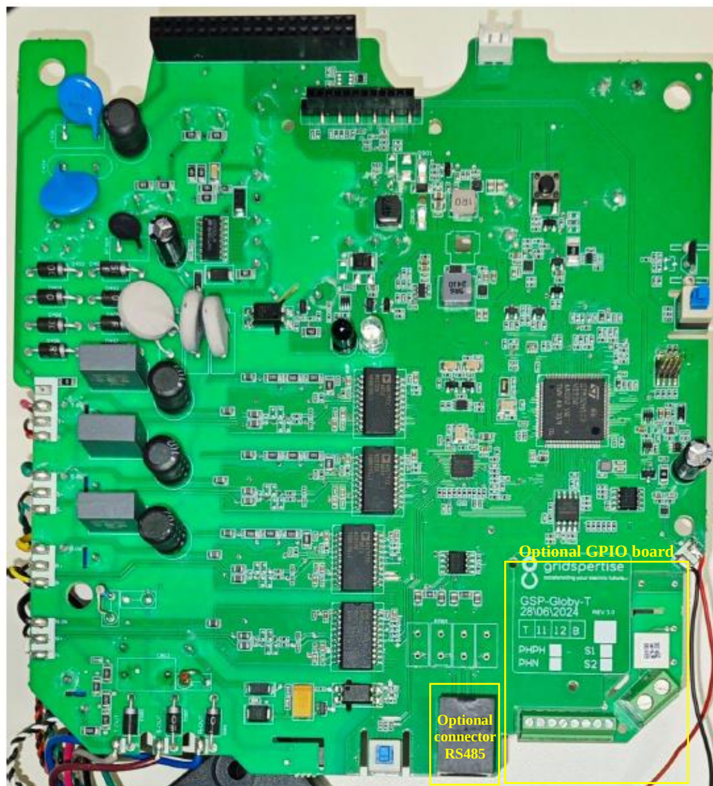
Figure 3 - GLOBYTGNG3 top PCB open view full version
