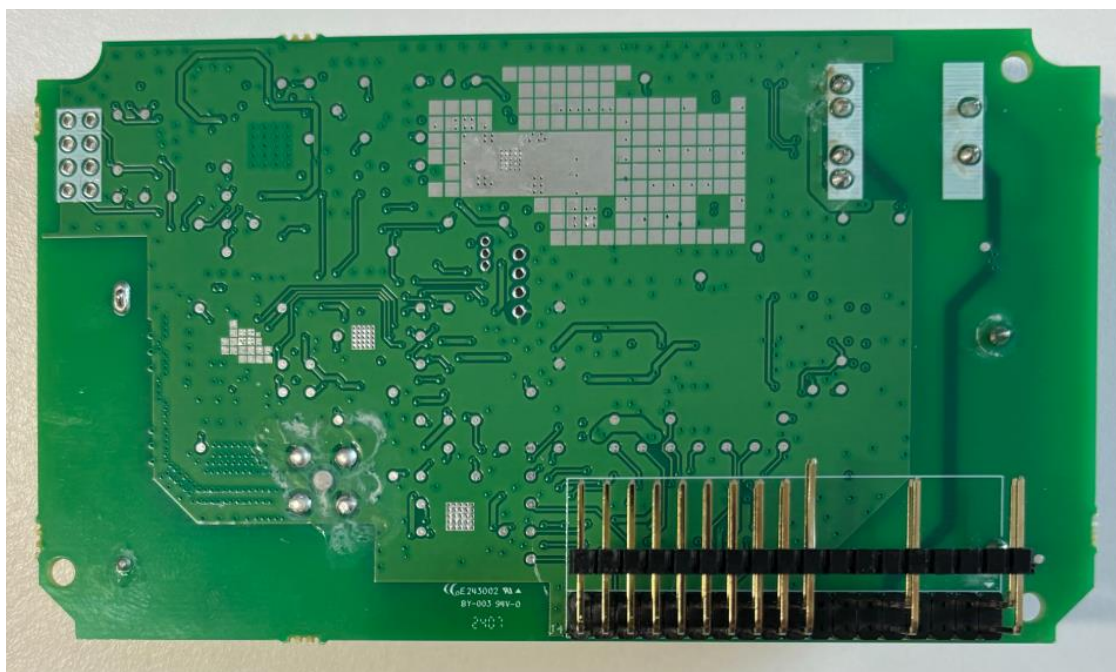
Figure 7 - GLOBYTNG3 communication module bottom view
