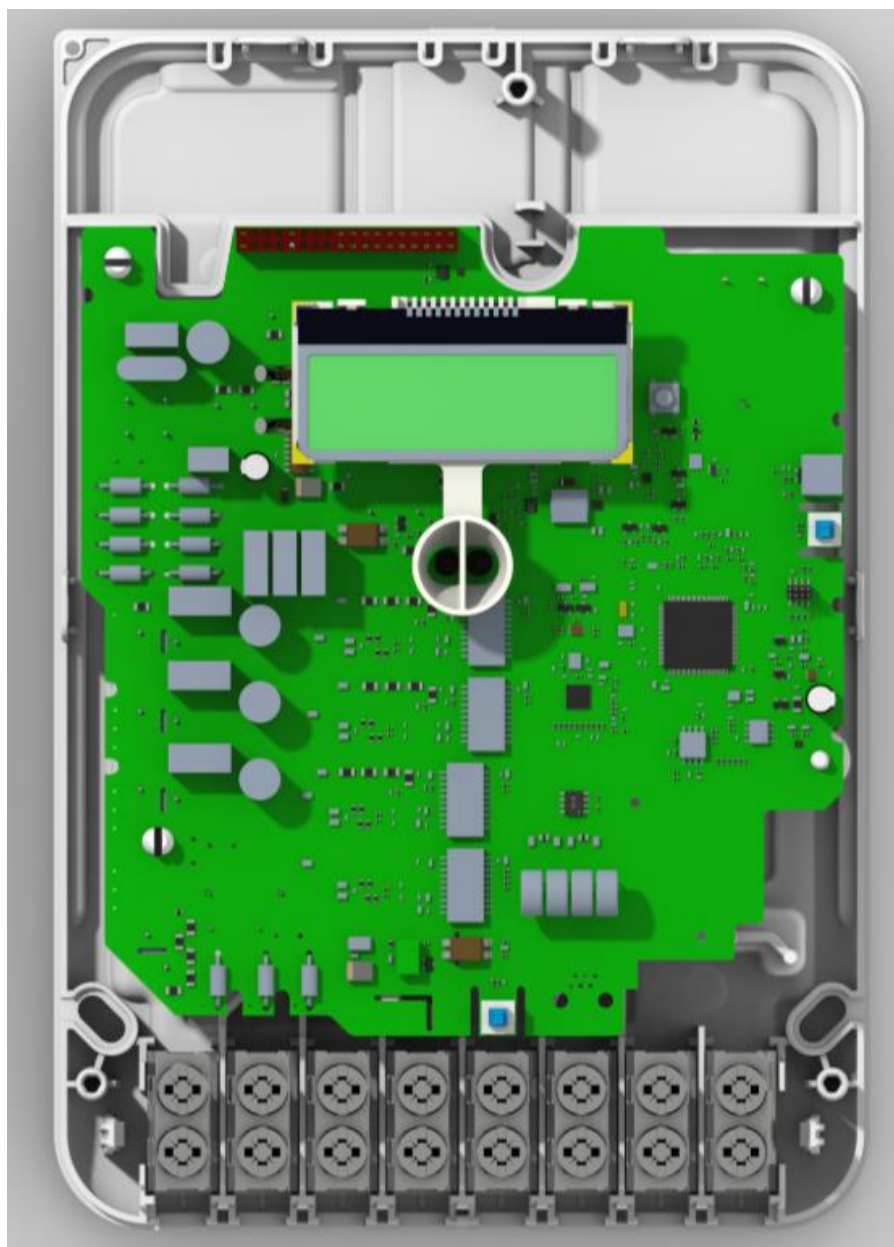
Figure 5 - Rendering of GLOBYTNG3 basic version top view
