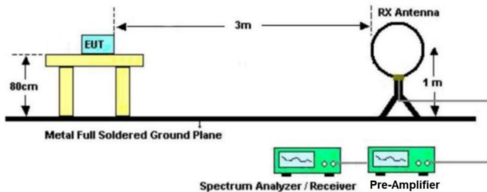
Figure 1. Below 30MHz
