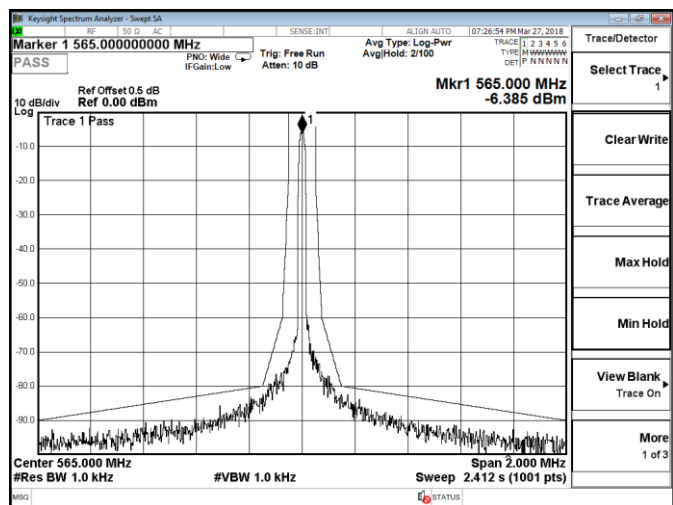
Channel 0 / 565 MHz
