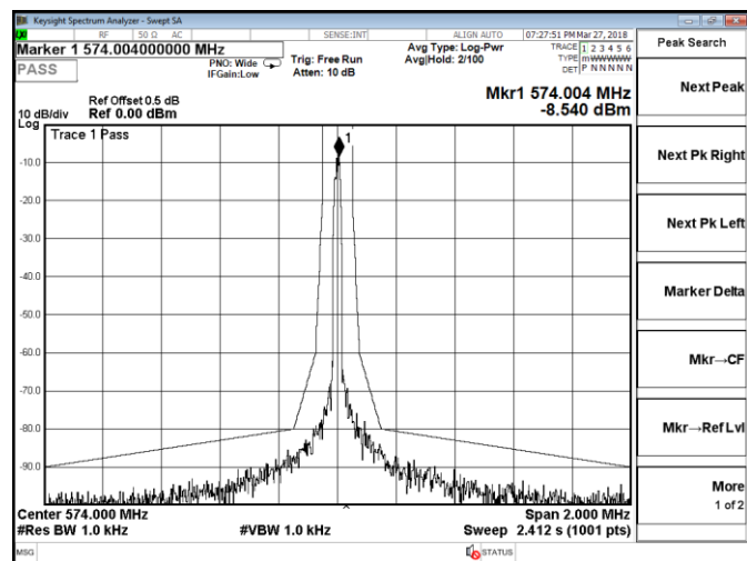
Channel 09 / 574 MHz
