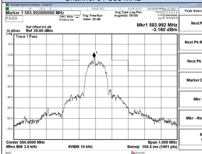
Channel 19 / 584 MHz
