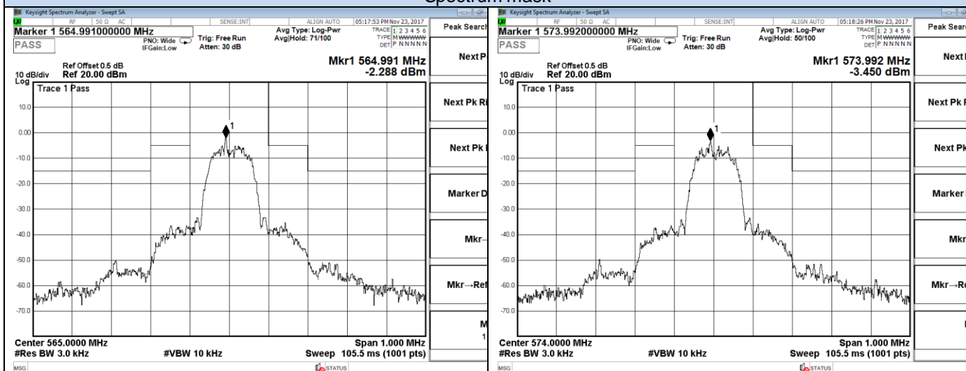
Channel 0 / 565 MHz
