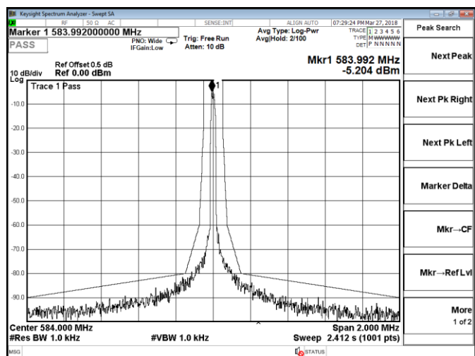
Channel 19 / 584 MHz
