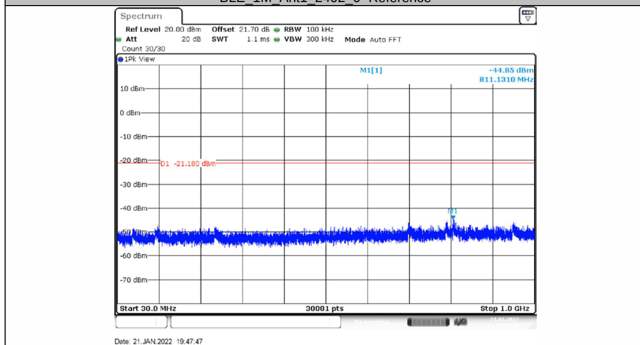
BLE_1M_Ant1_2402_30~1000
