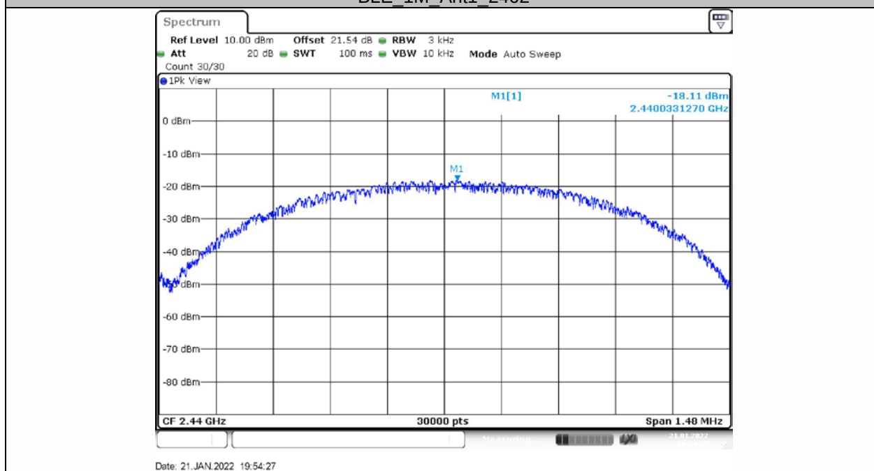
BLE_1M_Ant1_2440
