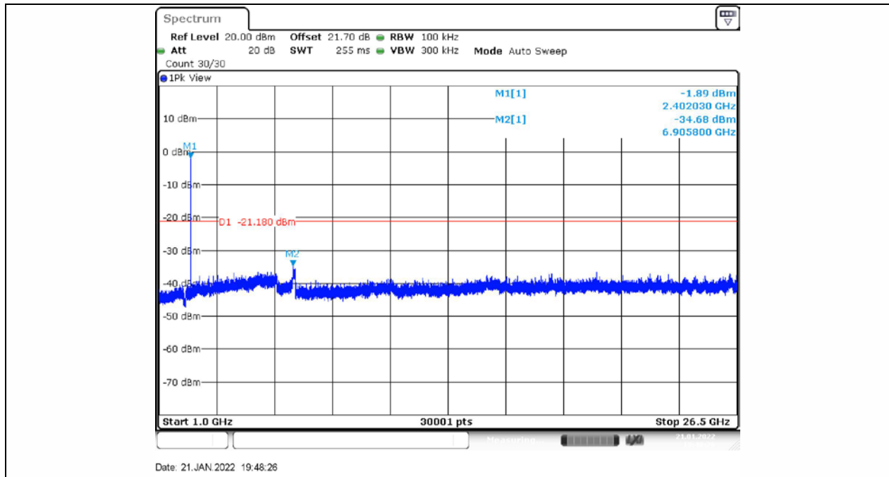
BLE_1M_Ant1_2402_1000~26500
