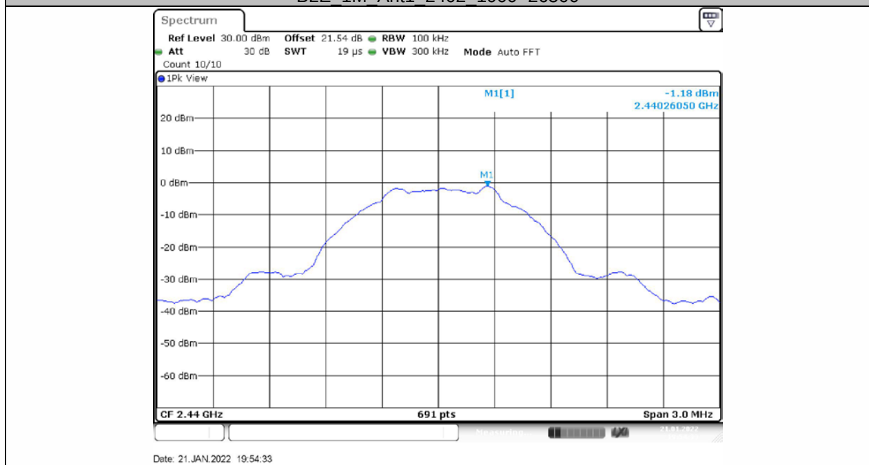
BLE_1M_Ant1_2440_0~Reference
