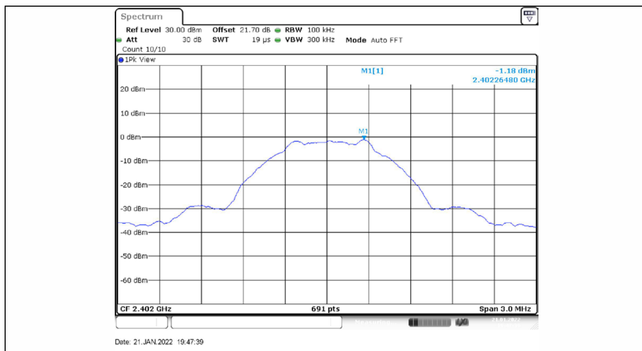
BLE_1M_Ant1_2402_0~Reference
