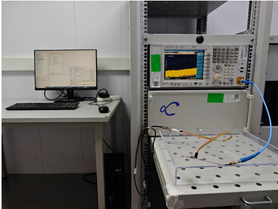
Conducted Test-LoRa
