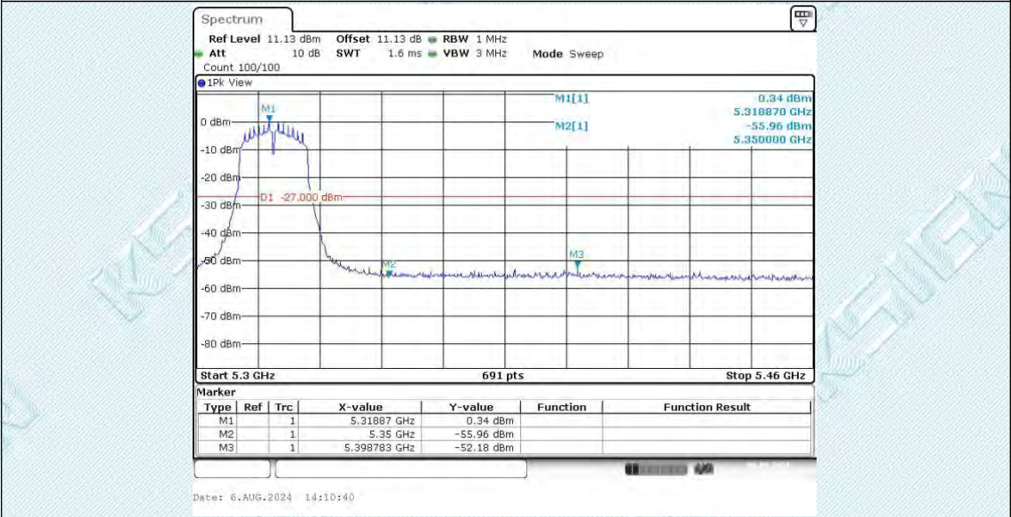
11N20SISO_Ant1_High_5320
