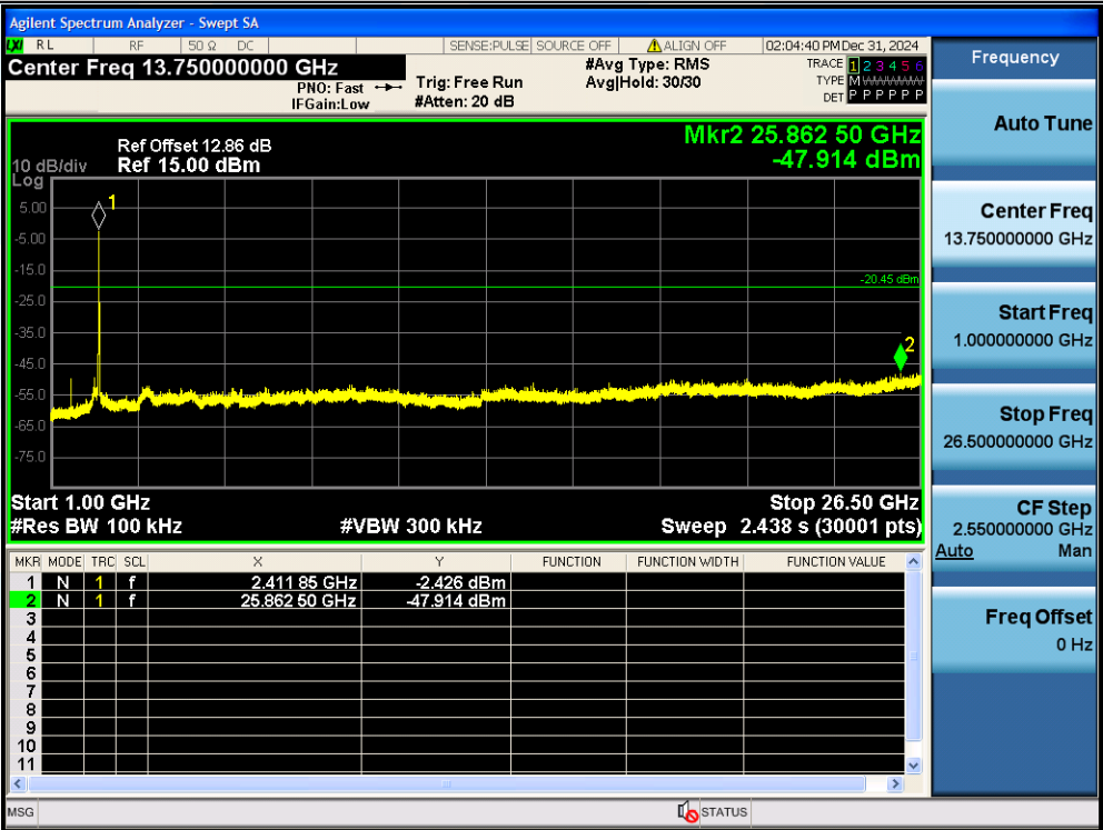
11G-Ant1-2412-1000~26500-PASS
