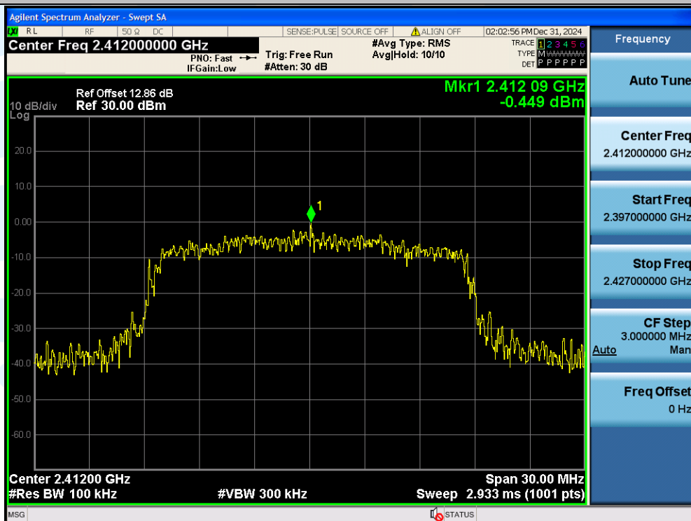
11G-Ant1-2412-0~Reference-PASS
