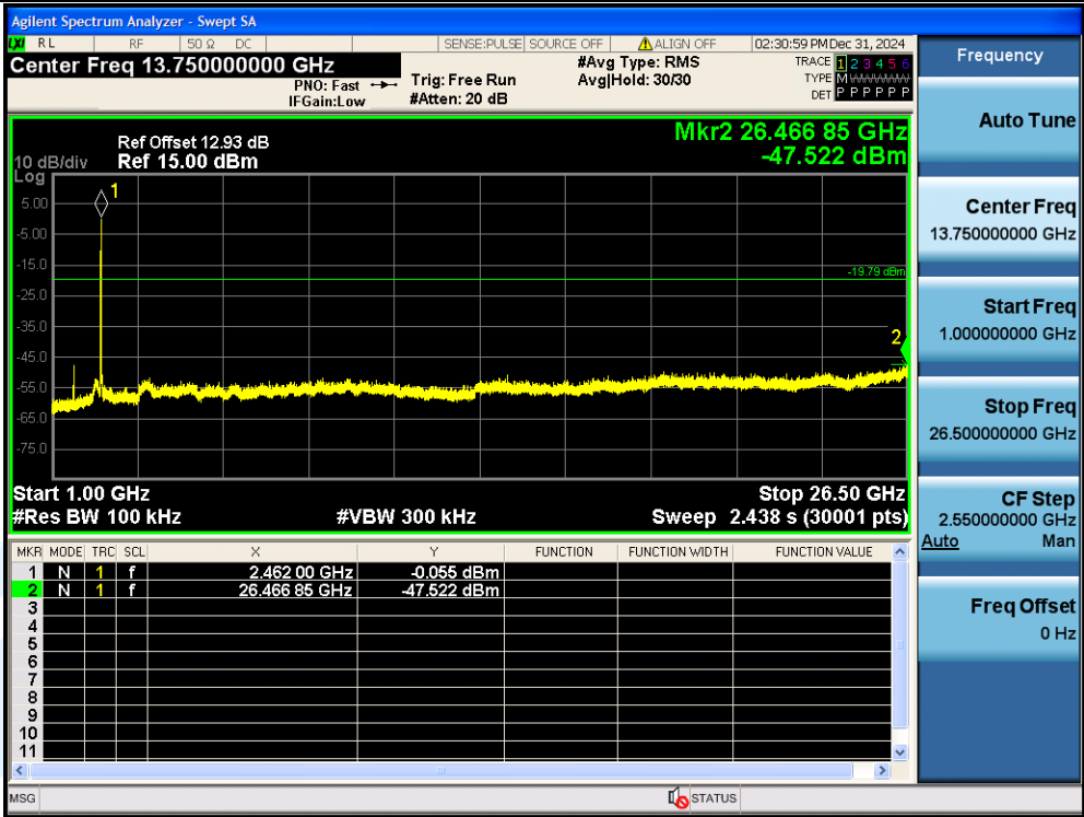
11N20SISO-Ant1-2462-1000~26500-PASS
