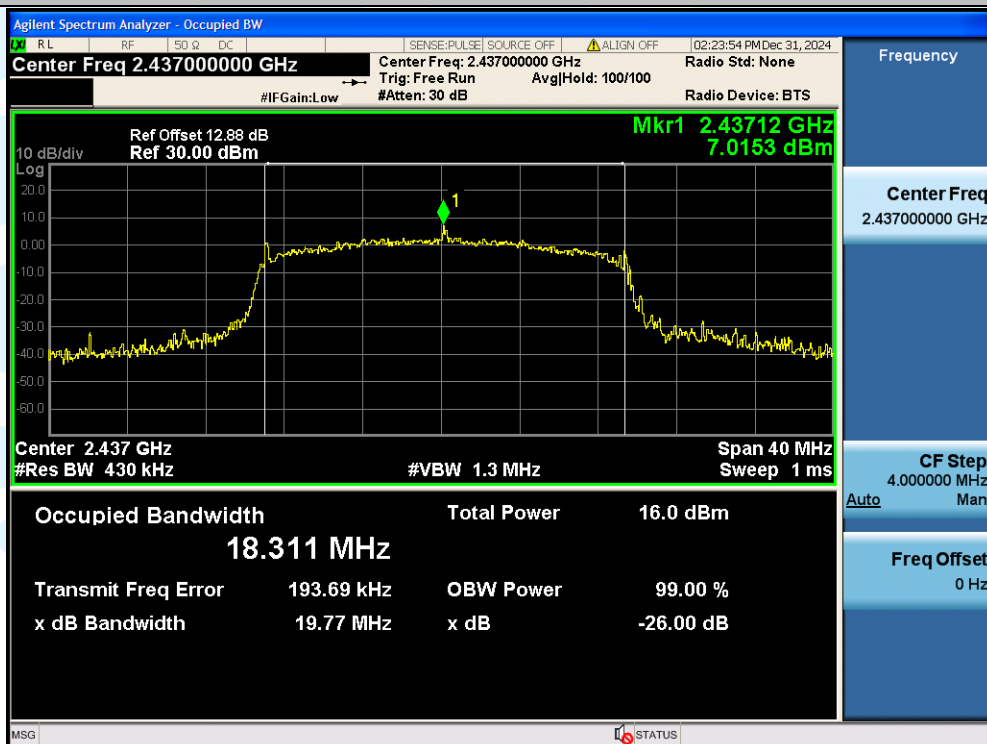
11N20SISO-Ant1-2437
