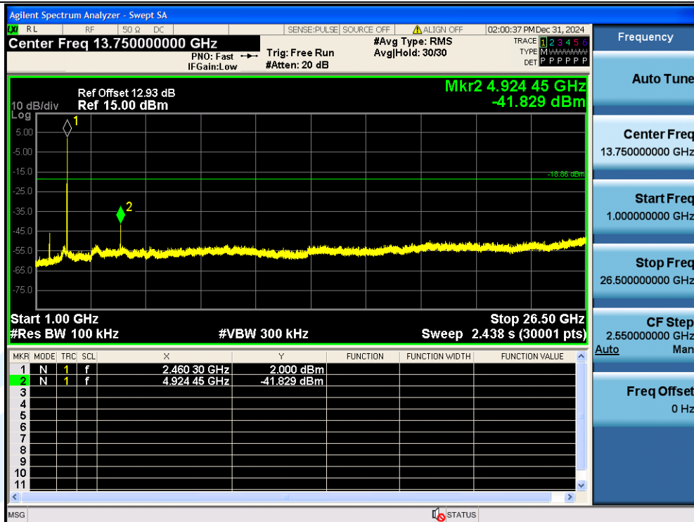
11B-Ant1-2462-1000~26500-PASS
