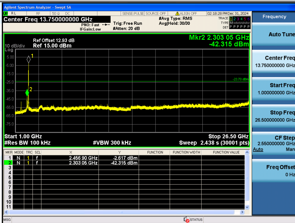
11G-Ant1-2462-1000~26500-PASS
