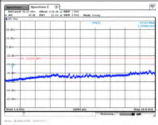
3 MHz / QPSK - Hight / CH21640 / 1RB5 / Above 1 GHz
