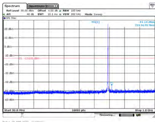
10 MHz / QPSK / CH134092 / 1RB0 / Below 1 GHz
