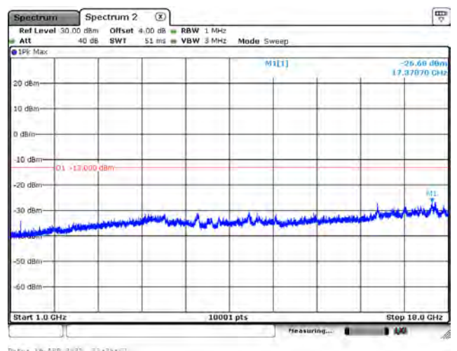
10 MHz / QPSK / CH134092 / 1RB0 / Above 1 GHz
