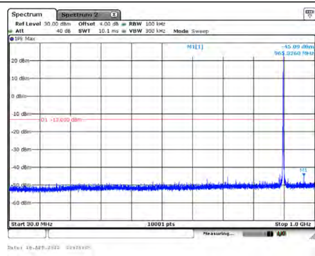
3 MHz / QPSK - Hight / CH21640 / 1RB5 / Below 1 GHz
