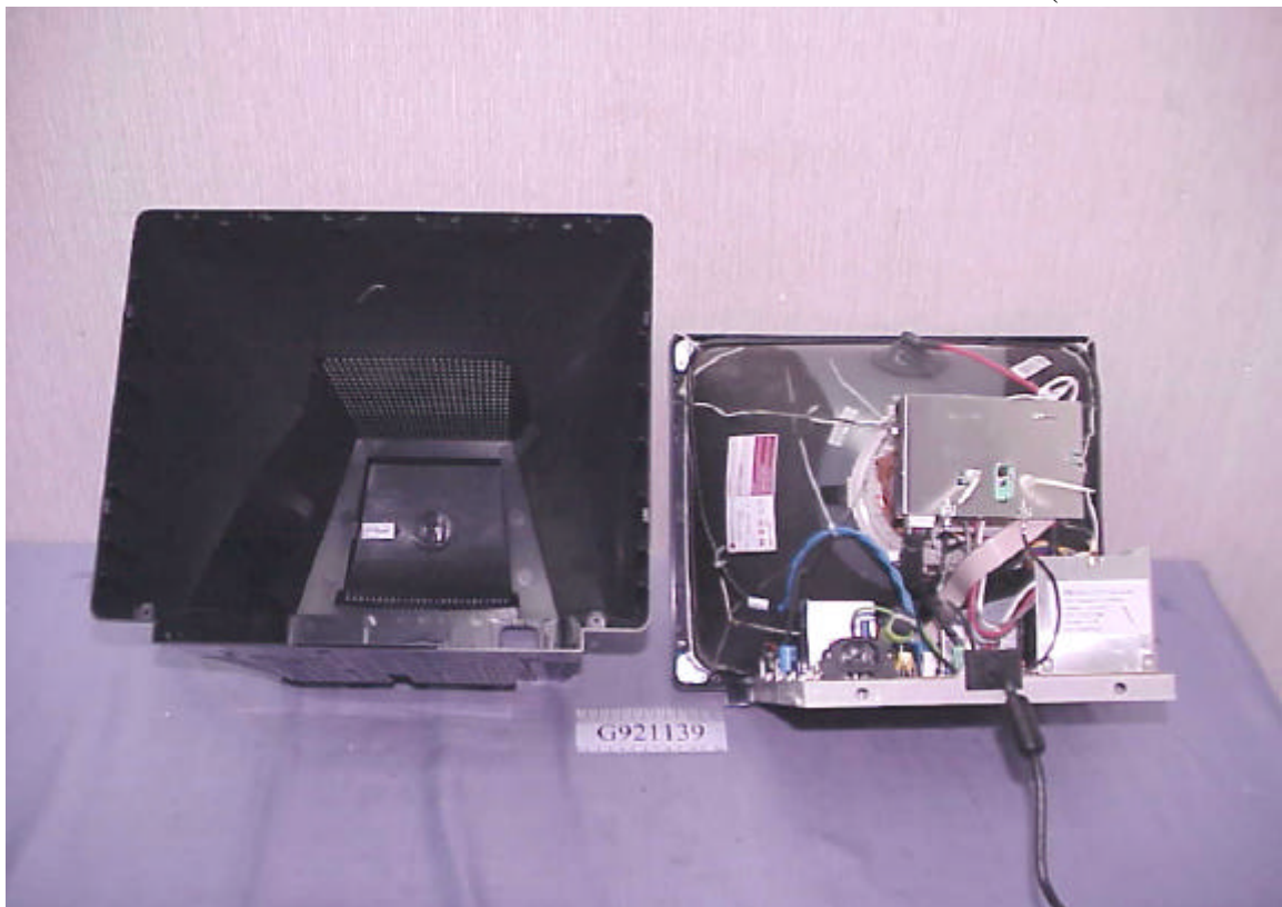
Figure 6 Display Color Monitor Internal View (Back Cover Removed)
