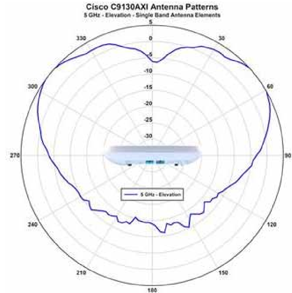
Figure 3-10 C9130AXI - Single-band Antenna radiation pattern (5 GHz Elevation)
