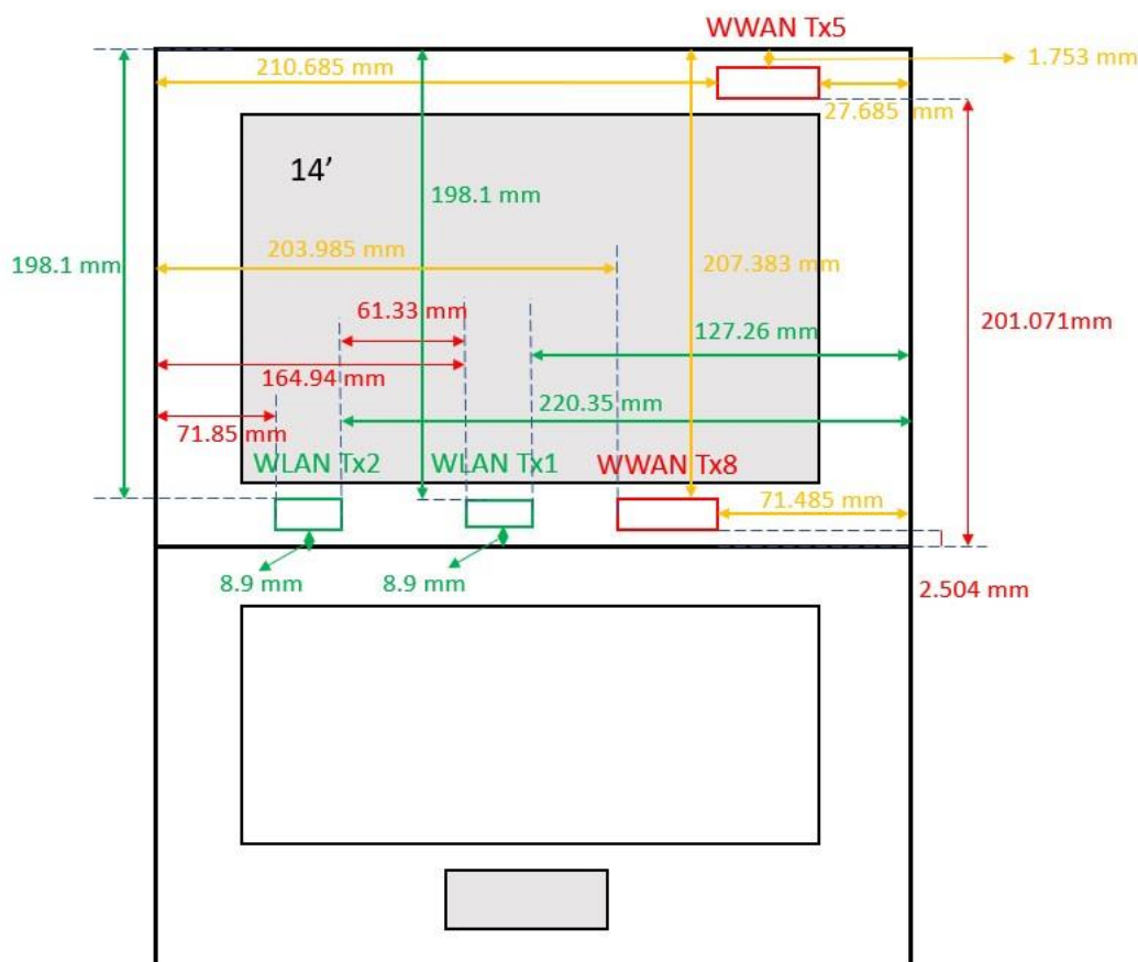
Fig.6 Antenna position of EUT
