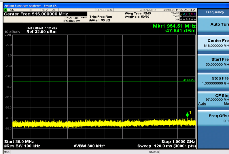
Band2-15MHz-64QAM-18675-1RB#0-30~1000MHz
