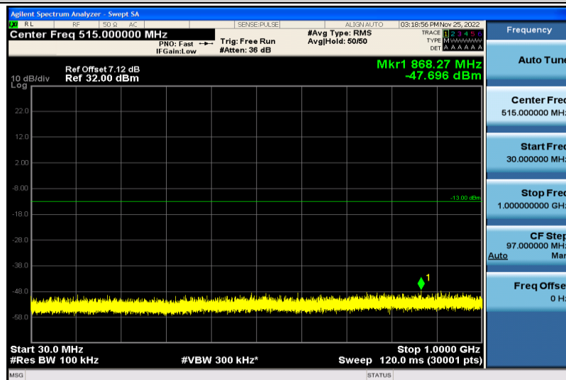
Band4-1.4MHz-64QAM-19957-1RB#0-30~1000MHz
