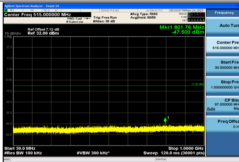
Band4-5MHz-QPSK-19975-1RB#0-30~1000MHz
