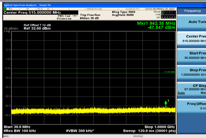
Band4-3MHz-64QAM-19965-1RB#0-30~1000MHz
