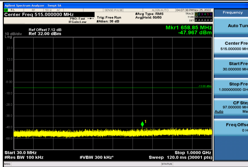
Band4-5MHz-64QAM-20175-1RB#0-30~1000MHz
