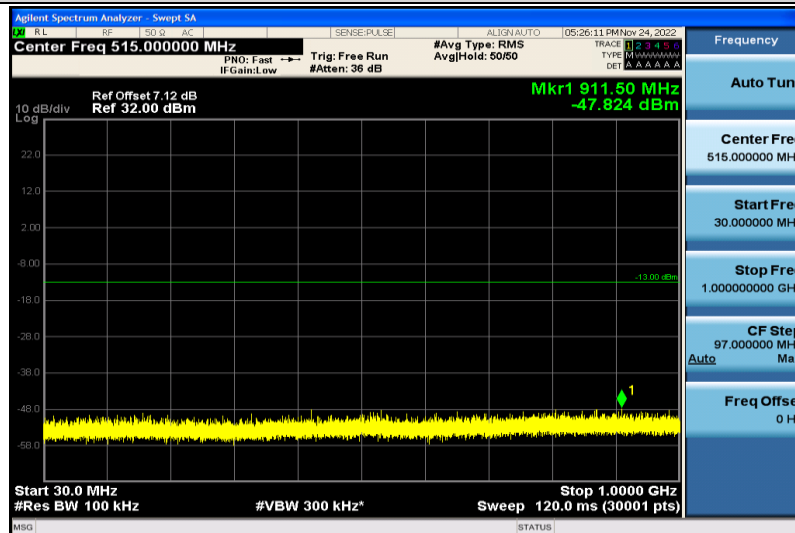
Band4-5MHz-16QAM-20375-1RB#0-30~1000MHz
