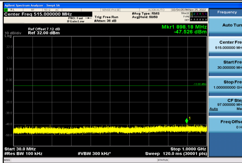
Band4-3MHz-64QAM-20175-1RB#0-30~1000MHz
