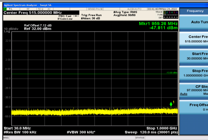
Band2-15MHz-16QAM-18675-1RB#0-30~1000MHz
