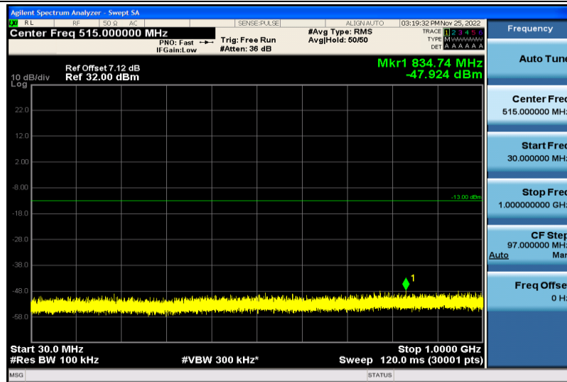
Band4-1.4MHz-64QAM-20175-1RB#0-30~1000MHz
