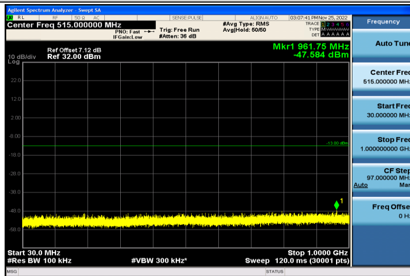
Band2-20MHz-64QAM-18700-1RB#0-30~1000MHz
