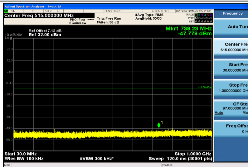
Band2-15MHz-64QAM-19125-1RB#0-30~1000MHz
