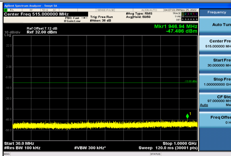
Band4-5MHz-64QAM-19975-1RB#0-30~1000MHz
