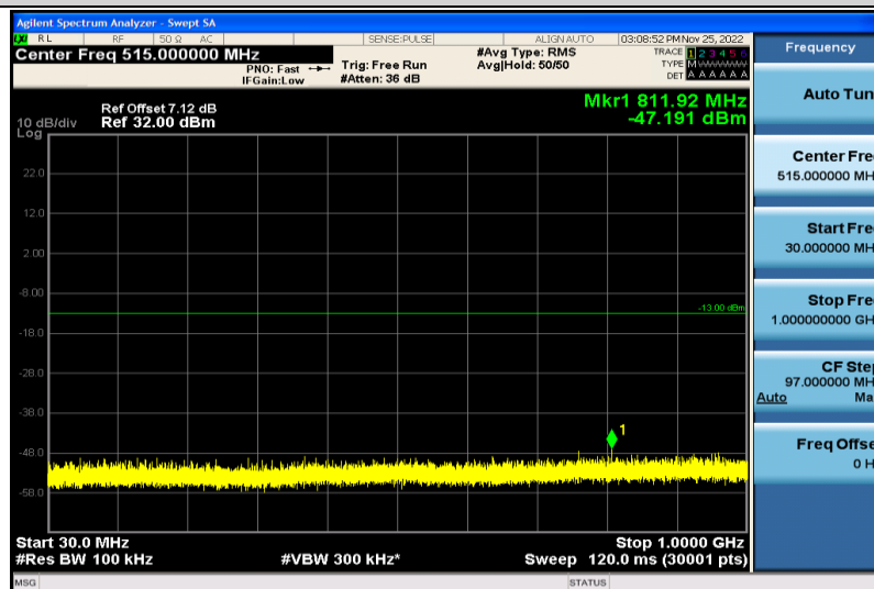
Band2-20MHz-64QAM-19100-1RB#0-30~1000MHz
