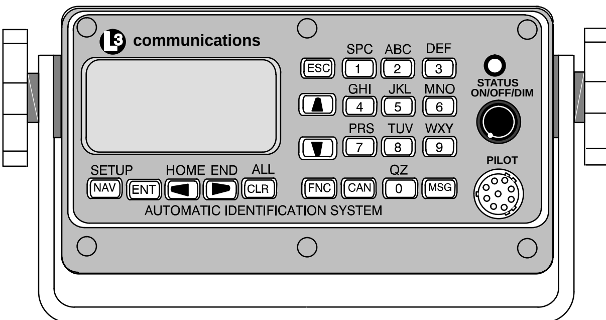
Figure 2–1. AIS Transponder
