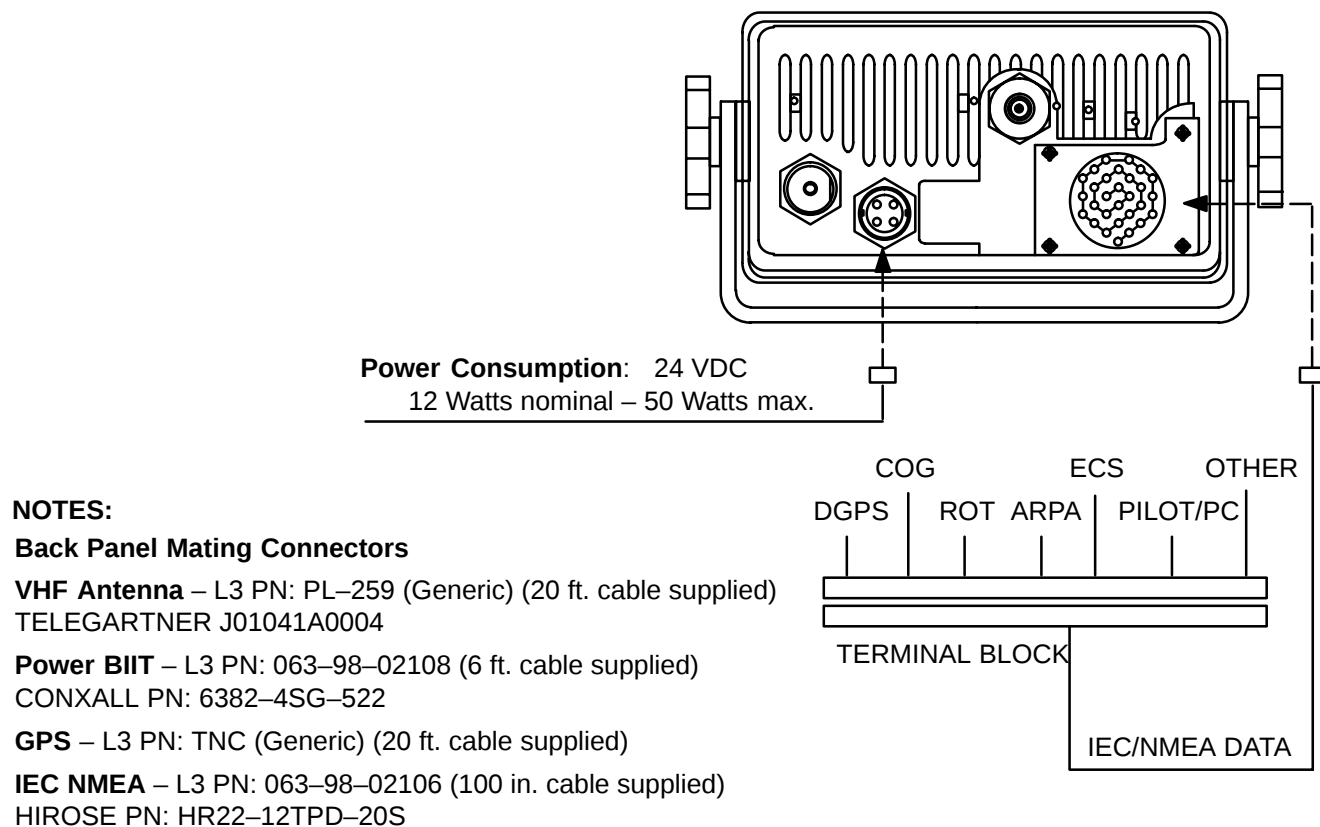
Figure 3-6. AIS Transponder Rear View
