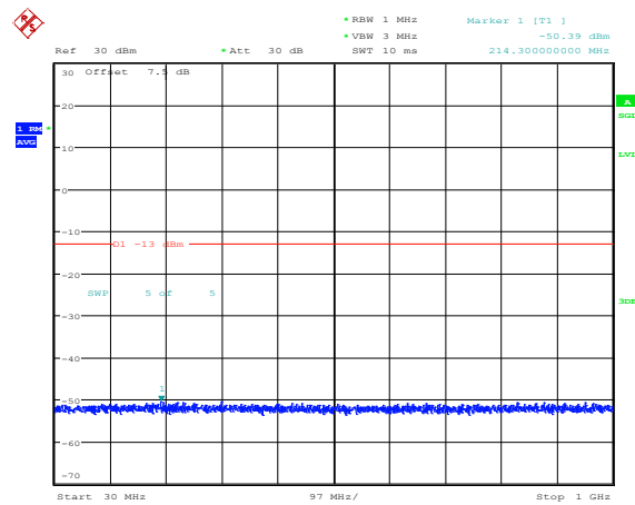
Band4-3MHz-16QAM-20385-1RB#0-Range3:30~1000MHz
