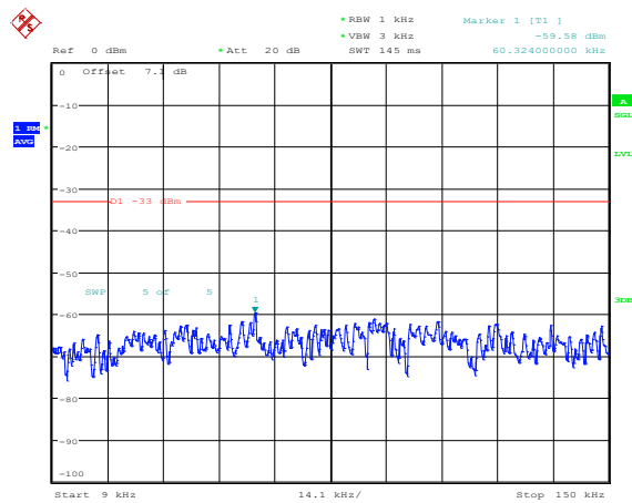
Band4-3MHz-QPSK-20175-1RB#0-Range1:0.009~0.15MHz
