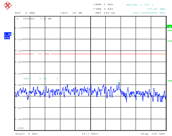
Band4-5MHz-16QAM-20175-1RB#0-Range1:0.009~0.15MHz
