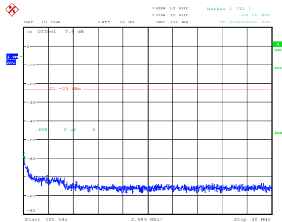
Band4-5MHz-16QAM-20175-1RB#0-Range2:0.15~30MHz
