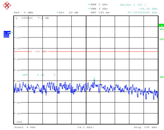
Band4-1.4MHz-16QAM-20175-1RB#0-Range1:0.009~0.15MHz
