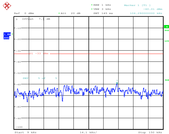
Band4-3MHz-QPSK-20385-1RB#0-Range1:0.009~0.15MHz
