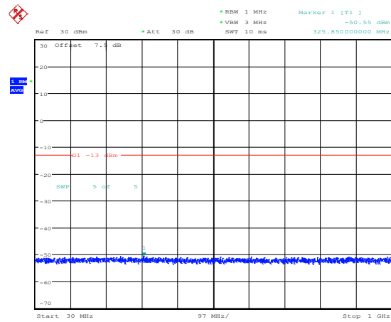
Band4-10MHz-16QAM-20350-1RB#0-Range3:30~1000MHz
