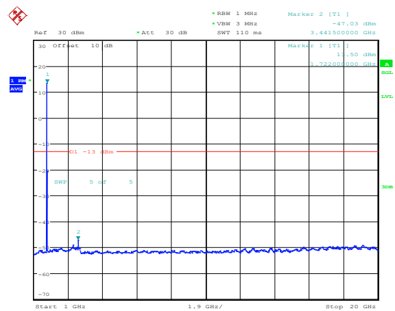
Band4-20MHz-16QAM-20175-1RB#0-Range4:1000~20000MHz
