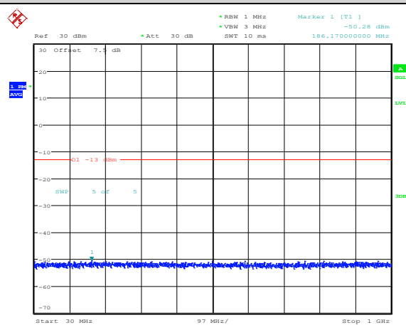
Band4-1.4MHz-QPSK-19957-1RB#0-Range3:30~1000MHz
