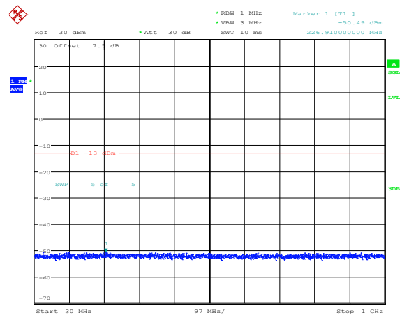
Band4-15MHz-QPSK-20025-1RB#0-Range3:30~1000MHz
