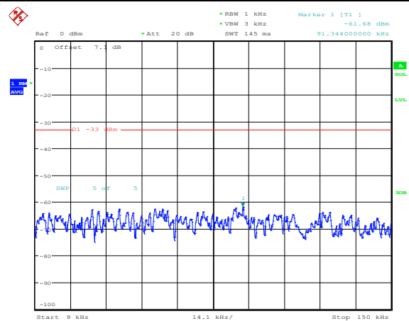
Band4-20MHz-16QAM-20300-1RB#0-Range1:0.009~0.15MHz
