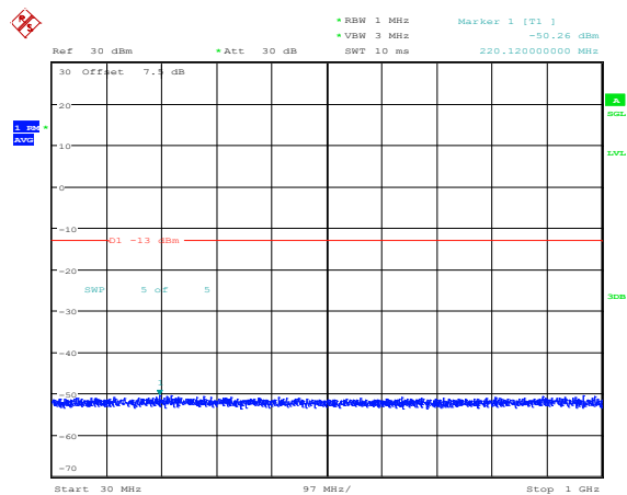
Band4-10MHz-16QAM-20000-1RB#0-Range3:30~1000MHz
