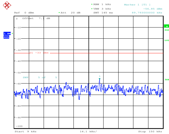
Band4-15MHz-QPSK-20175-1RB#0-Range1:0.009~0.15MHz
