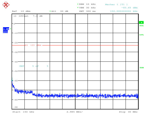
Band4-10MHz-16QAM-20000-1RB#0-Range2:0.15~30MHz
