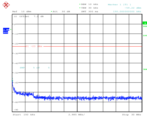
Band4-15MHz-QPSK-20175-1RB#0-Range2:0.15~30MHz
