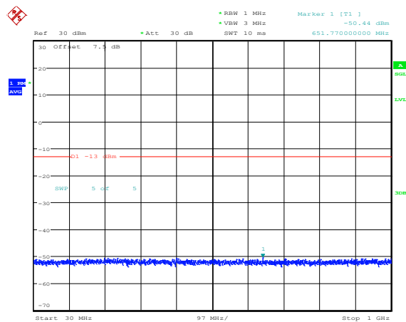
Band4-20MHz-16QAM-20050-1RB#0-Range3:30~1000MHz
