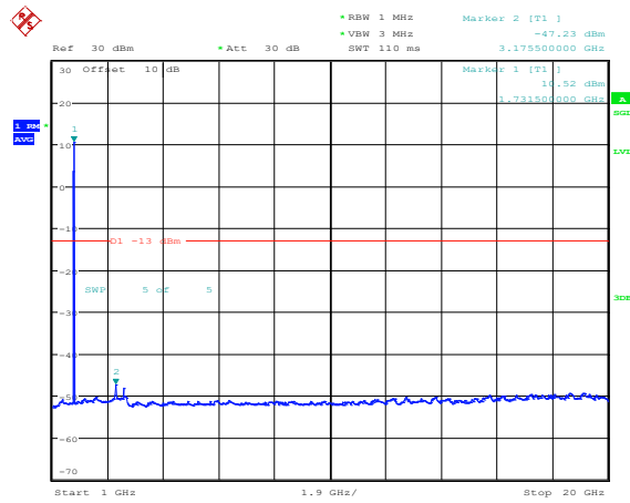
Band4-3MHz-16QAM-20175-1RB#0-Range4:1000~20000MHz
