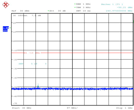
Band4-15MHz-QPSK-20325-1RB#0-Range3:30~1000MHz
