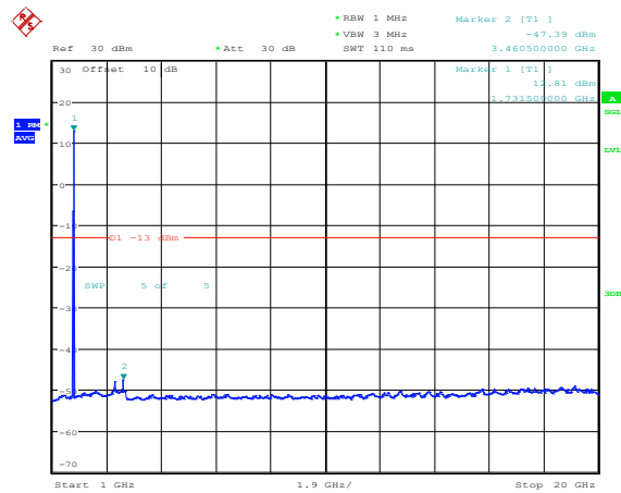
Band4-1.4MHz-16QAM-20175-1RB#0-Range4:1000~20000MHz
