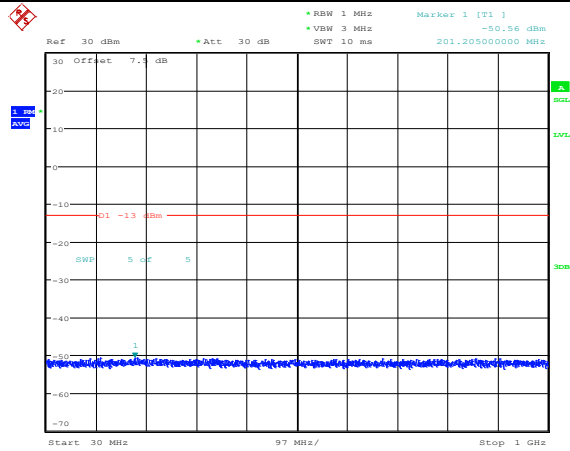
Band4-1.4MHz-QPSK-20393-1RB#0-Range3:30~1000MHz
