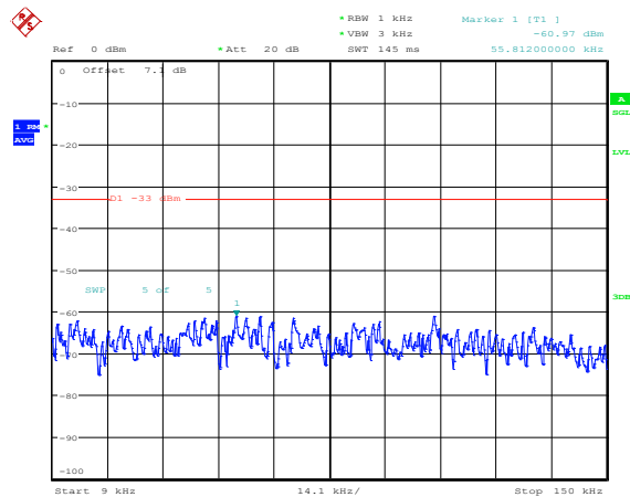
Band4-10MHz-16QAM-20350-1RB#0-Range1:0.009~0.15MHz
