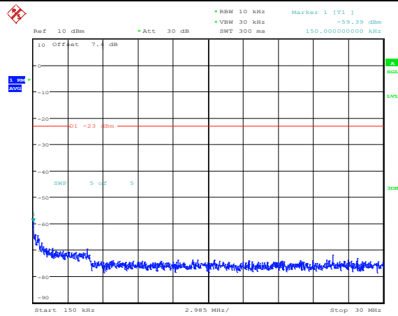
Band4-20MHz-16QAM-20050-1RB#0-Range2:0.15~30MHz
