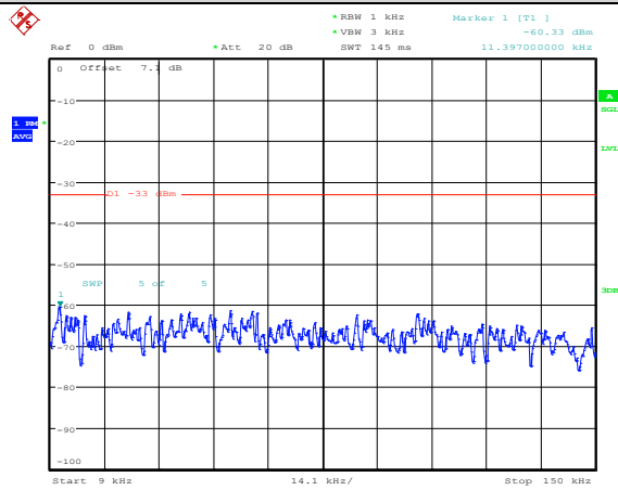
Band4-3MHz-16QAM-20385-1RB#0-Range1:0.009~0.15MHz
