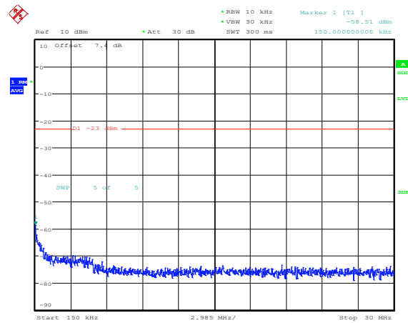
Band4-1.4MHz-16QAM-20175-1RB#0-Range2:0.15~30MHz
