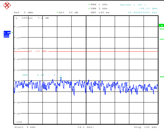
Band4-1.4MHz-16QAM-20393-1RB#0-Range1:0.009~0.15MHz
