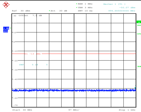
Band4-5MHz-QPSK-20375-1RB#0-Range3:30~1000MHz
