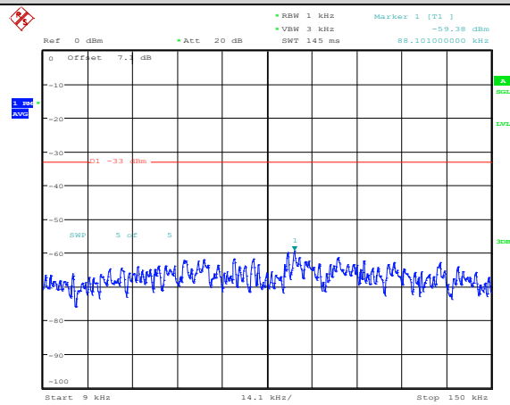
Band4-1.4MHz-QPSK-19957-1RB#0-Range1:0.009~0.15MHz
