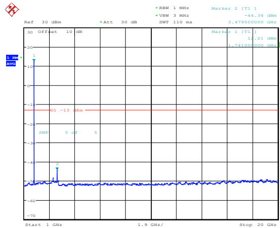
Band4-15MHz-QPSK-20325-1RB#0-Range4:1000~20000MHz
