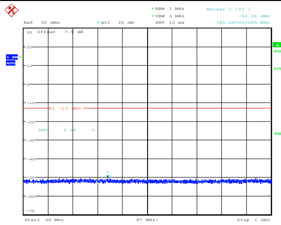
Band4-20MHz-QPSK-20300-1RB#0-Range3:30~1000MHz
