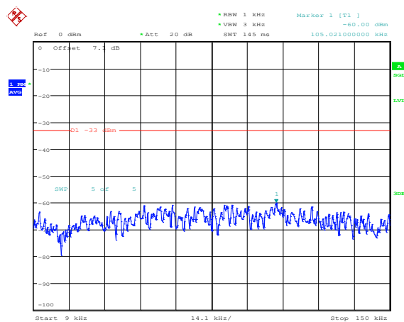
Band4-20MHz-QPSK-20300-1RB#0-Range1:0.009~0.15MHz
