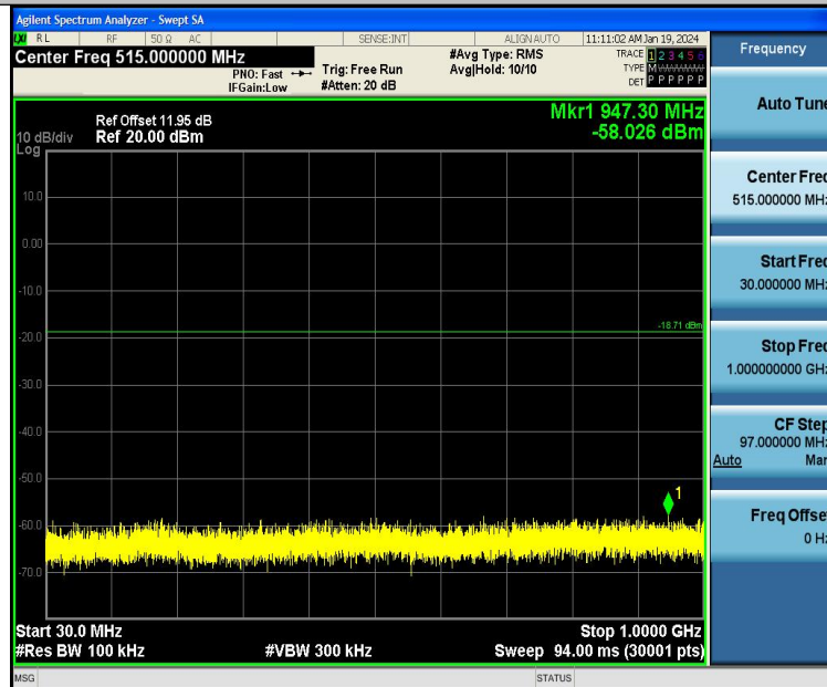
11B-Ant1-2412-30~1000-PASS
