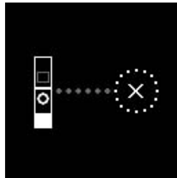
Connection Failure
