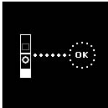
Connection Successful
