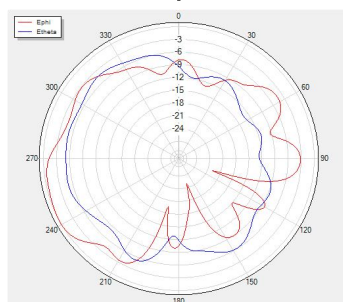
Phi=90 freq=2400MHz
