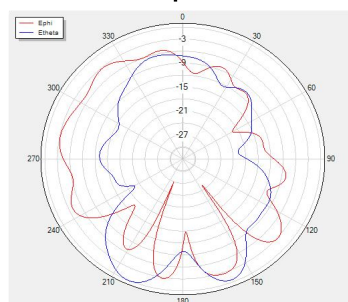
Phi=0 freq=2400MHz
