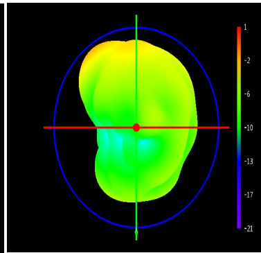
Phi=0 freq=2400MHz
