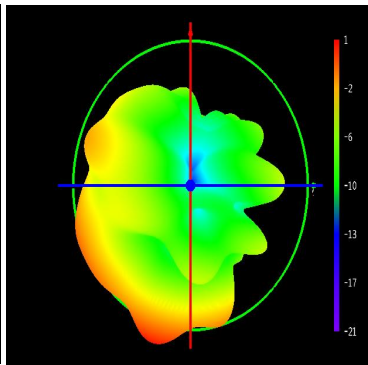
Phi=90 freq=2400MHz
