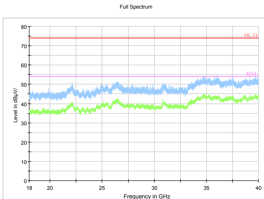
Pic13. Radiated emission (18GHz –40GHz)
