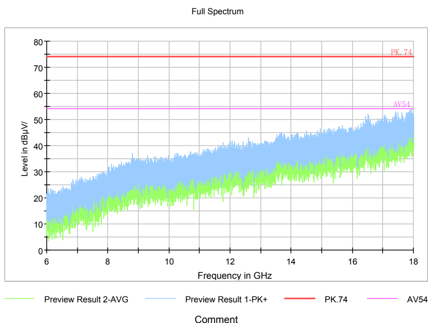
Pic12. Radiated emission (6GHz –18GHz)
