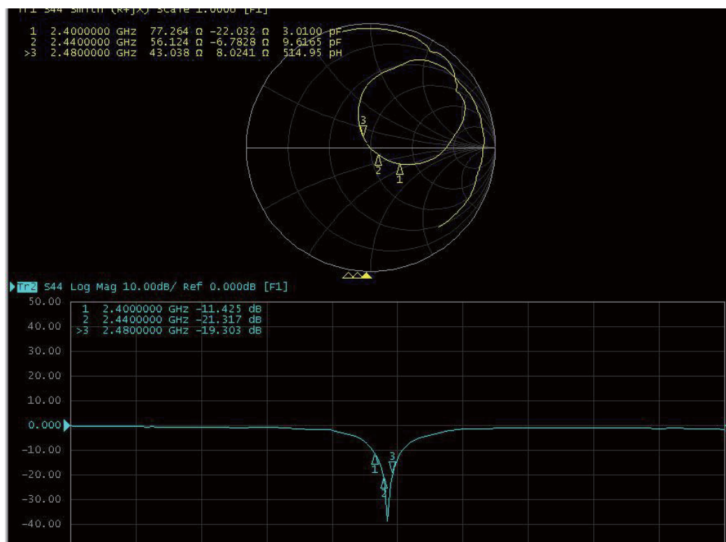
Return Loss
