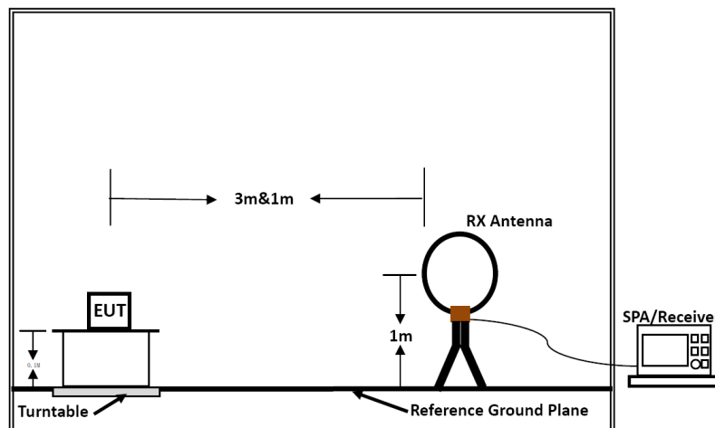
Below 30MHz
