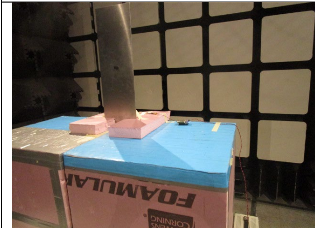
Radiated Emissions – Y orientation
