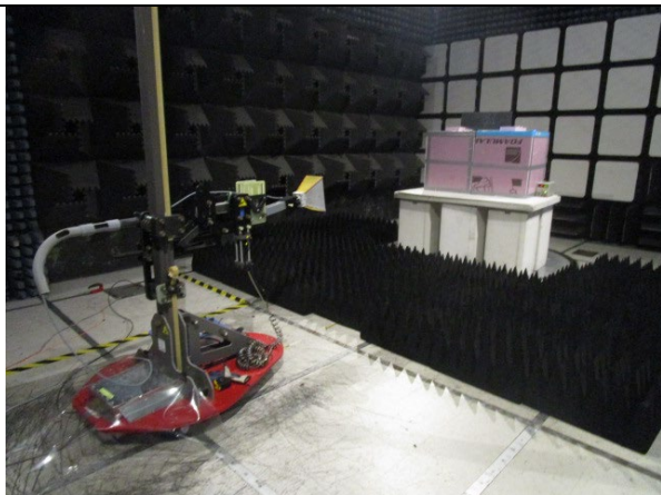
Radiated Emissions – Front
