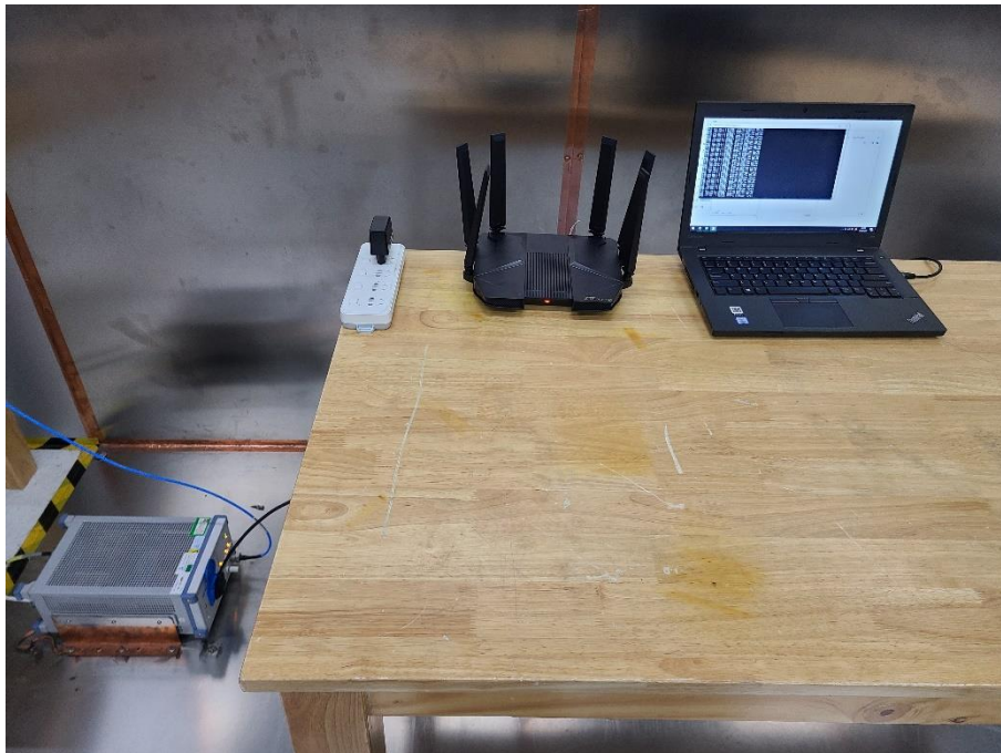
Photograph 4: Set-up photo for Conducted Emission
