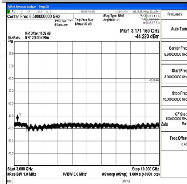
Band5_10MHz_QPSK_20450_1RB#0_3000~10000_300 0~10000
