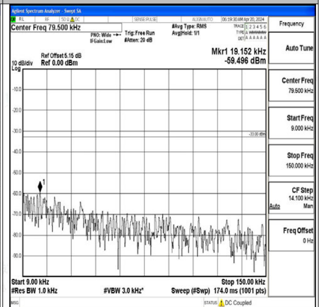
Band5_10MHz_16QAM_20450_1RB#0_0.009~0.15_0.0 09~0.15
