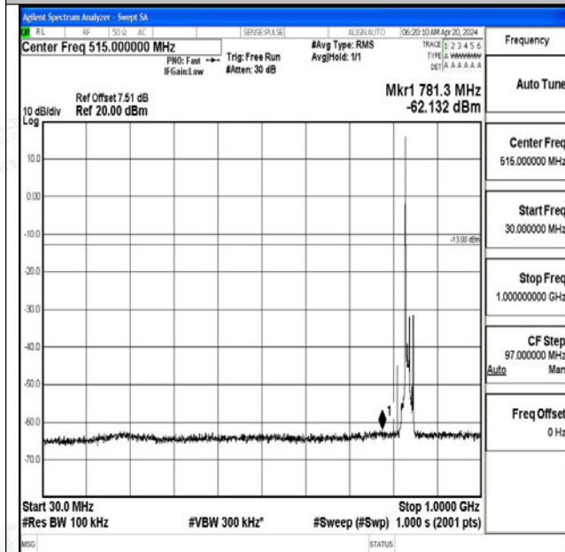
Band5_10MHz_QPSK_20525_1RB#0_30~1000_30~1000
