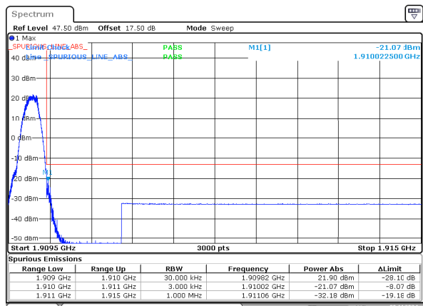
GSM_High
