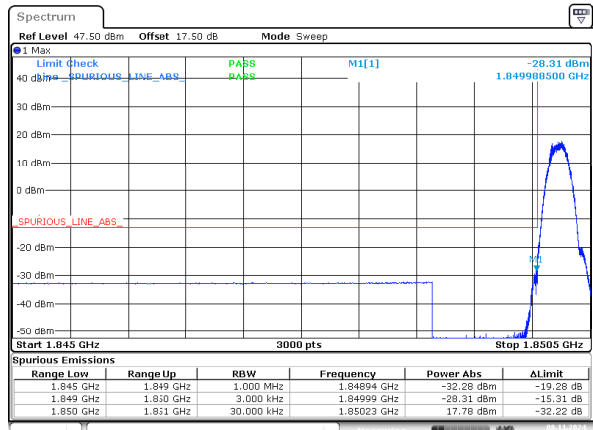
EDGE_Low_Solt1
