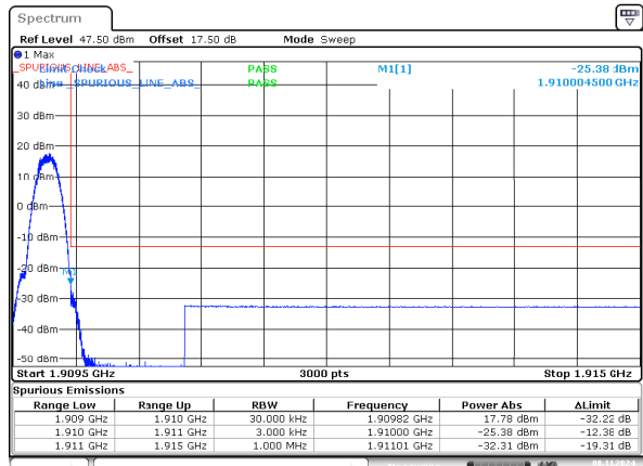
EDGE_High_Solt1
