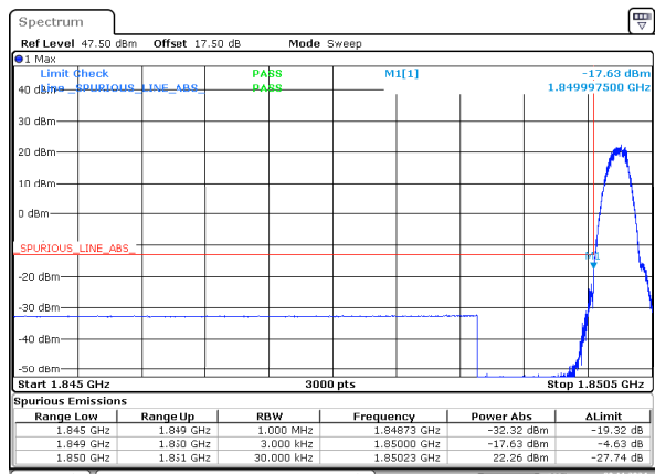
GSM_Low
