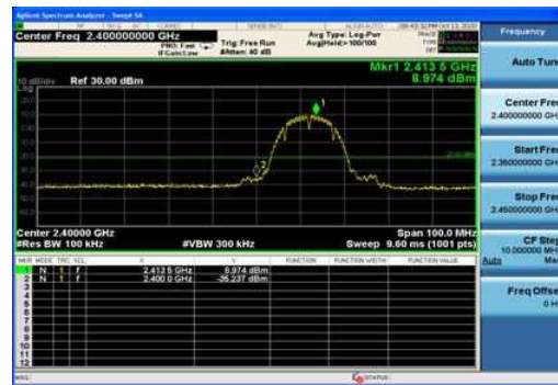
802.11g, Channel No.: 1
