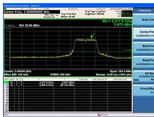
802.11n(HT40), Channel No.: 3
