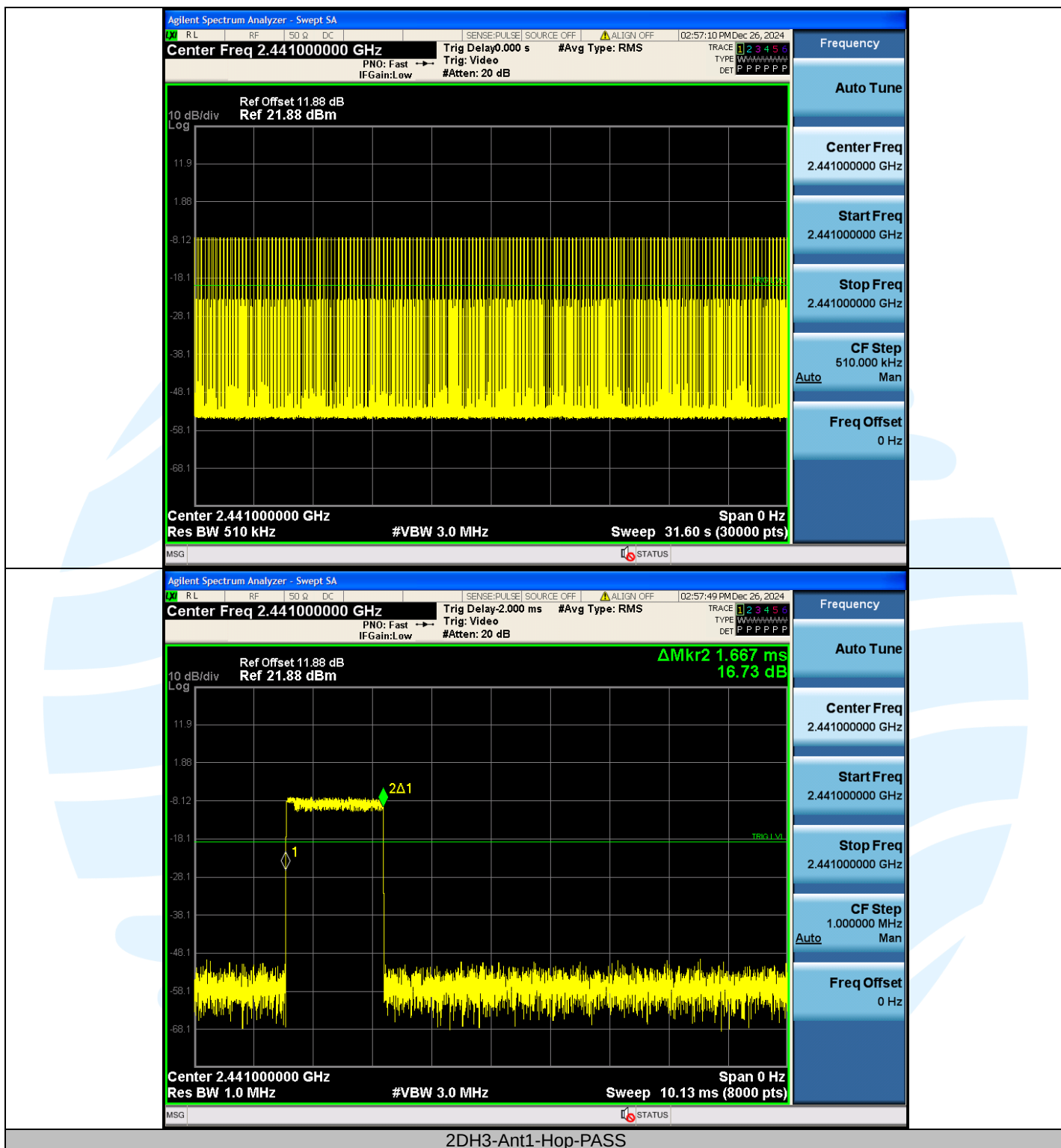
2DH3-Ant1-Hop-PASS
