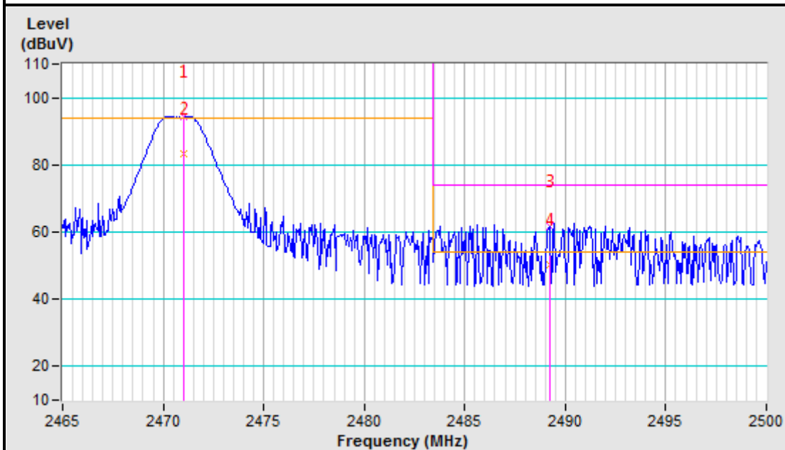
2483.5MHz Vertical
