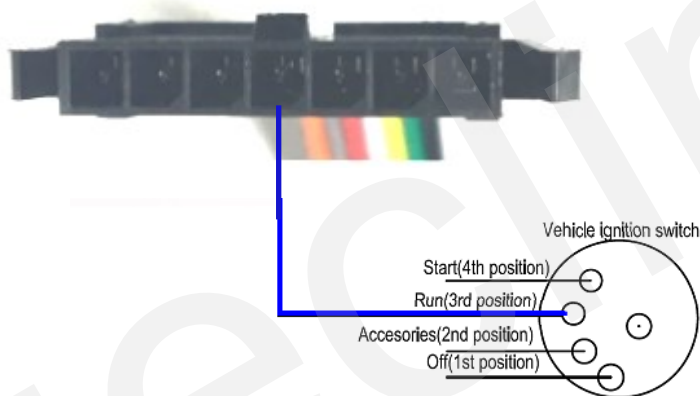
Figure 4: Typical Ignition Detection
