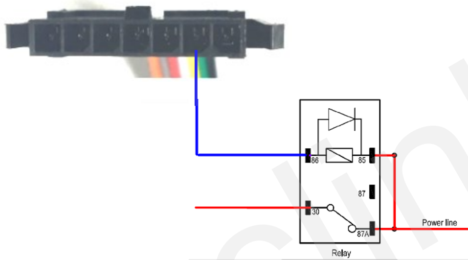
Figure 9: Typical Connection with Relay
