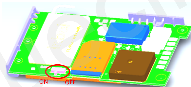
Figure 4. Switch and ON/OFF Position
