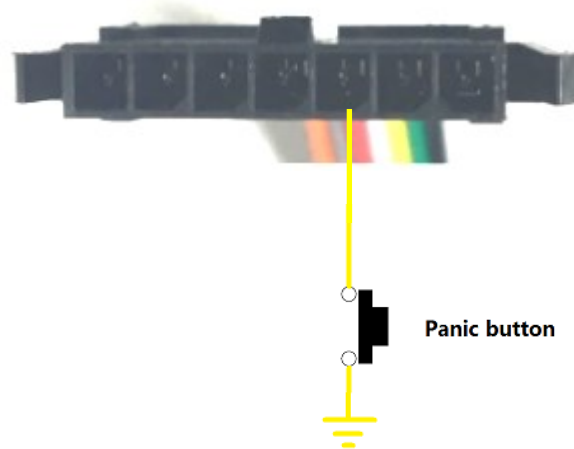
Figure 7: Typical Digital Input Connection
